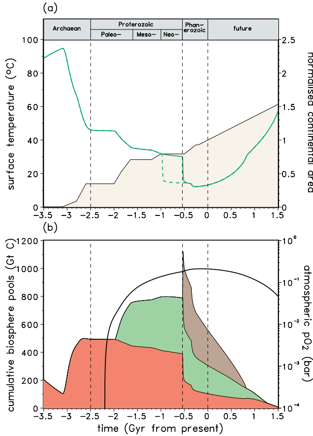
Figure 1. (a) Evolution of global surface temperature (solid green line). The green dashed line denotes a second possible evolutionary path triggered by a temperature perturbation in the Neoproterozoic era. The colored area indicates the evolution of the normalized continental area according to Condie [1990]. (b) Evolution of the cumulative biosphere pools for procaryotes (red), eucaryotes (green), and complex multicellular life (brown). The solid black curve denotes the evolution of atmospheric pO_2 .
