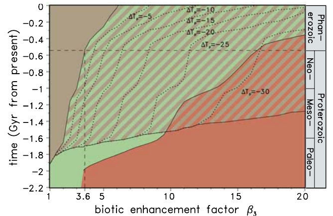
Figure 3. Stability diagram for the three types of biosphere as a function of the biotic enhancement factor, \beta_3 . In the red area only procaryotic life exists while in the green area eucaryotic and procaryotic life coexist. In the brown area complex multicellular life appears additionally. The dashed area indicates the time interval in which a cooling event may trigger the first emergence of complex multicellular life prematurely. The dotted lines denote the boundaries for certain amplitudes of temperature perturbations, \Delta T_p .
