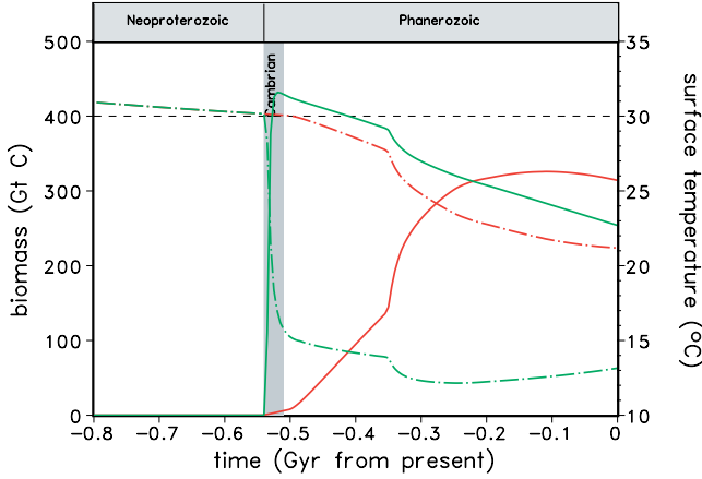
Figure 2. Evolution of the complex multicellular life biomass (solid lines) and the corresponding surface temperatures (dashed dotted lines). The green curves denote the results with enabled geosphere-biosphere feedback while the red curves denote the results for a disabled feedback. The horizontal dashed line indicates the upper temperature limit for the productivity of complex multicellular life ( T_{\max,3} ).
