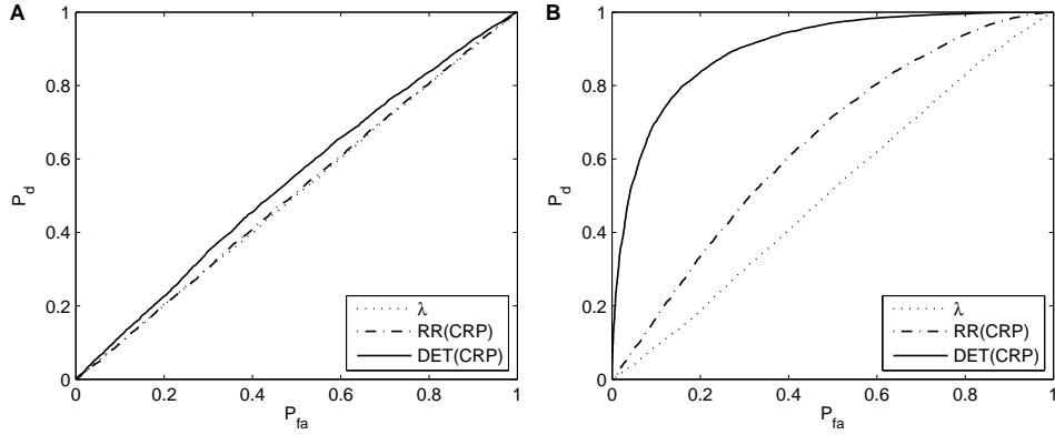
Fig. 2. ROC for the measures \lambda , RR and DET for the detection of a deterministic signal from white Gaussian noise. The signal used here is a harmonic signal s(t) = \cos(20t + \phi) , using a sampling interval of \Delta t = 0.01 , data length N = 1,000 and 10,000 realisations (the same result can be achieved using \Delta t = 1 ). The SNR is (A) 0.1 and (B) 0.5; the embedding parameters are m = 2 , \tau = 15 and the RP threshold \varepsilon = 1 .
