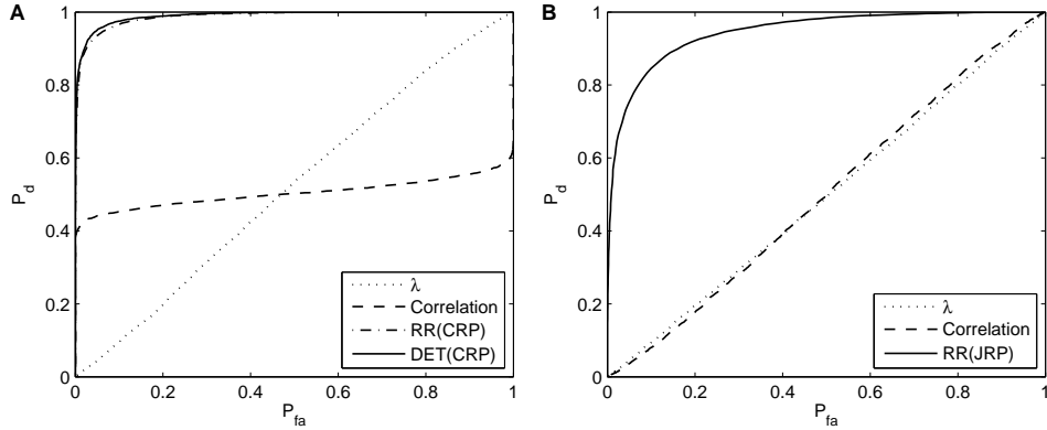
Fig. 4. (A) ROCs for the correlation receiver, the measure \lambda and the RQA measures RR and DET derived from a CRP for the detection of a noise corrupted signal from noise using a probe signal (SNR=0.5). The incoming signal x consists of the original signal s plus noise \xi . (B) ROCs for the correlation receiver, the measure \lambda and the RQA measure RR derived from a JRP (SNR=0.3). Here the signal s exists as a transformation of the measured signal x ( x = s^2 + \xi ). In both cases the signal is a stochastic harmonic process s(t) = \cos(20t + \phi) with random phases \phi , using a sampling interval of \Delta t = 0.01 , data length N = 1,000 and 10,000 realisations. The embeddings parameters are m = 2 , \tau = 15 and the RP threshold \varepsilon = 1 (for the JRP such \varepsilon is chosen that the RR of the RP is 0.1).
