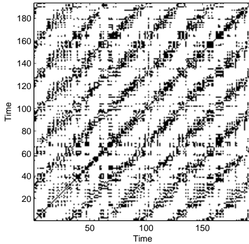
Fig. 3. Recurrence plot of the noise corrupted harmonic signal as used in Fig. 2 (SNR = 2). The embedding parameters are m = 2 , \tau = 8 and the RP threshold \varepsilon = 1 .
