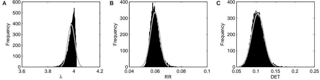
Fig. 1. Distributions of the measures (A) \lambda , (B) RR and (C) DET for 10,000 realisations of white Gaussian noise ( m = 2 , \tau = 2 , \varepsilon = 0.5 ). Fits of corresponding Gaussian distributions are shown (in gray).
