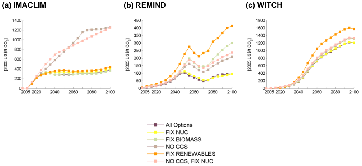
Figure 19: Carbon price trajectories for various technology constraint scenarios.
