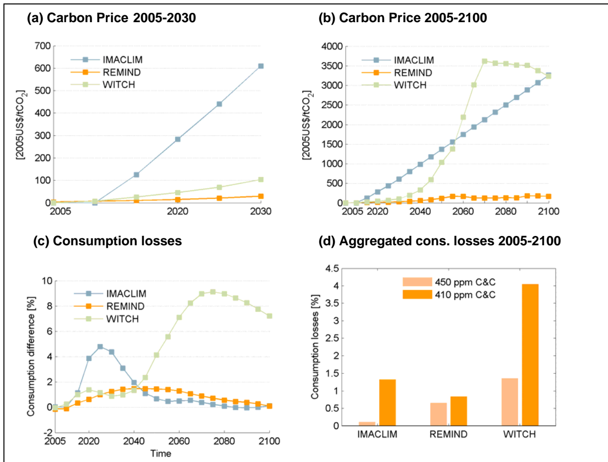
Figure 6: Carbon price (a,b), global consumption losses (c) for the 410 ppm stabilization scenario and comparison of aggregated consumption losses for the 410 and 450 ppm scenarios (d). Aggregated consumption losses are discounted by 3%.
