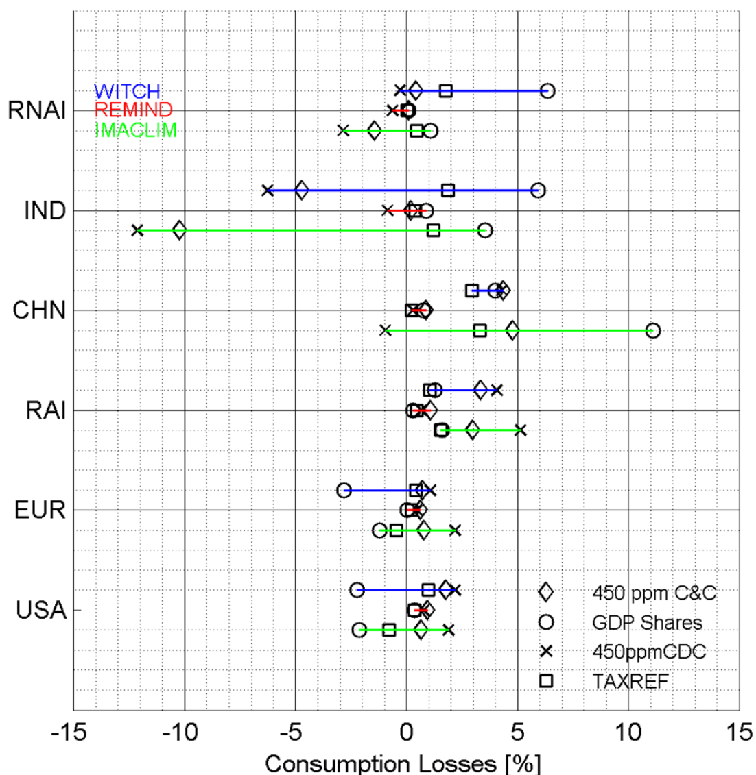
Figure 16: Distributional effects of various allocation schemes to achieve 450 ppm CO 2 in terms of consumption losses for the models IMACLIM-R, REMIND-R and WITCH. Percentage changes are given relative to baseline using a 3% discount rate.
