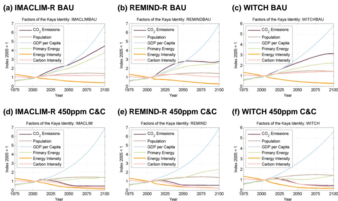
Figure 3: Kaya factors for the baseline and the 450 ppm C&C as projected by the RECIPE models (2005-2100). For comparison, historic trends based on IEA (2007) are depicted for 1975-2005.
