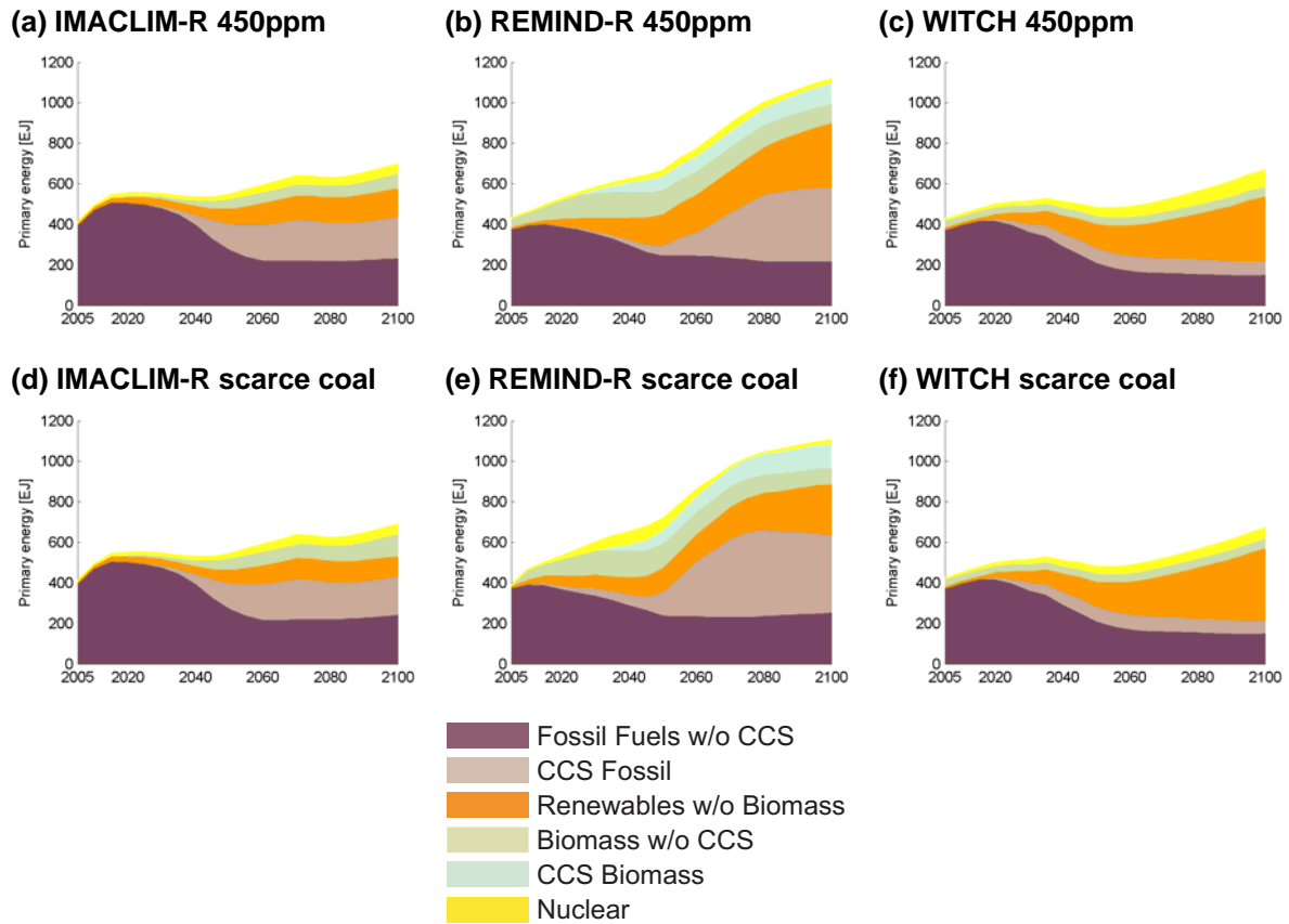
Figure 14: Sensitivity of energy mix to scarcer coal
