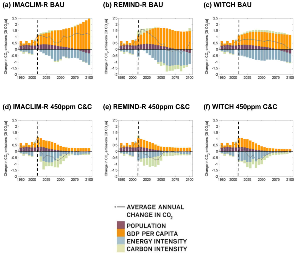
Figure 2: Decomposition of historic CO 2 emission trends and model results for IMACLIM-R, REMIND-R and WITCH for the baseline and the 450 ppm C&C scenario in terms of the driving factors population growth, per capita GDP, energy intensity of economic output, and carbon intensity of primary energy use. The dashed lines indicate the transition from historic data (IEA) to modeled data (RECIPE models). Note different scales between BAU and policy scenarios.
