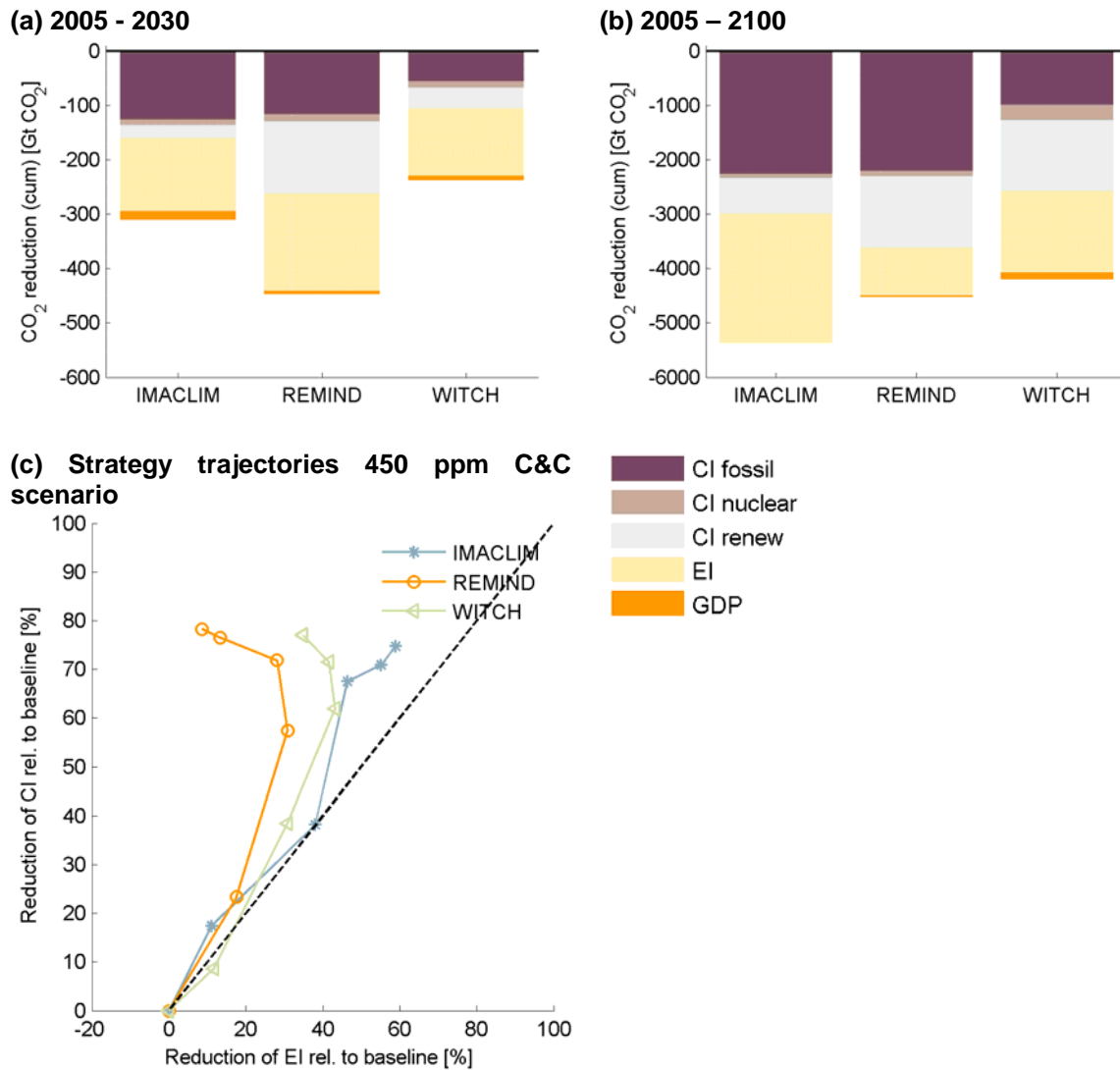
Figure 4: Relative contribution of energy and carbon intensity reduction to the required reduction in energy-related CO 2 -emissions for (a) 2005-2030 for the 450ppm C&C scenario, (b) the entire simulation period 2005-2100 for the 450ppm C&C scenario (c) the temporal evolution of carbon and energy intensity relative to baseline for the years 2005, 2020, 2040, 2060, 2080, and 2100 for the 450ppm C&C scenario.
