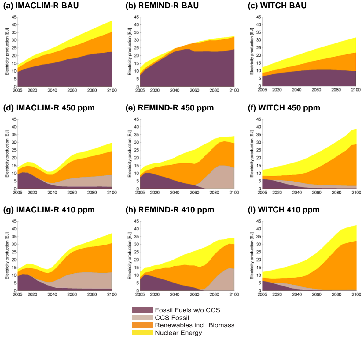
Figure 25: Electricity mix for the European power sector (IMACLIM-R and WITCH) as well as power and heat for REMIND-R
