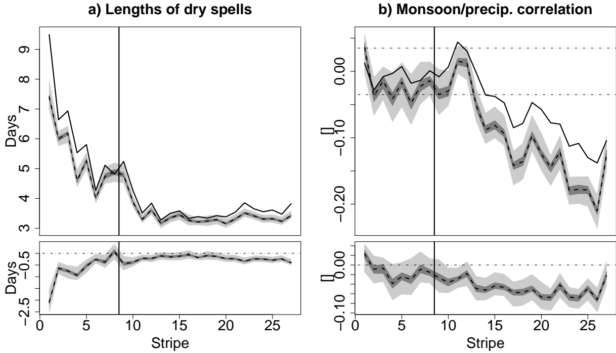
FIG. 6. a) Average dry spell lengths and b) correlation between monsoon strength (WNPMI) and daily precipitation along the Yangtze: profiles from the observation period (solid black line); spread (light gray shaded), inter-quartile range (dark gray shaded) and median (dashed black line) of the STAR ensemble projections. The dashed-dotted lines in the upper right panel indicate the 90%-confidence interval for the Null-hypothesis (Spearman's correlation coefficient equals 0, serial correlation taken into account). Bottom panel: Differences of future projections minus training period observations; shades and lines as in top panel.
