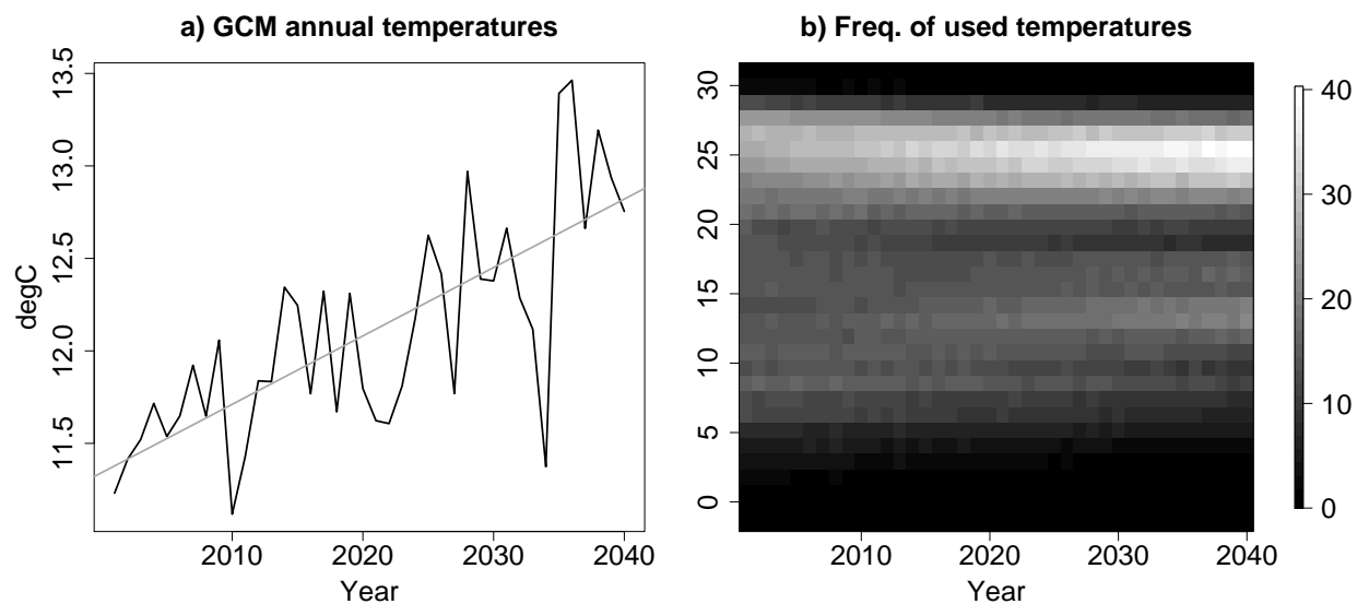
FIG. 2. a) ECHAM5 annual temperatures, averaged over the five grid cells which contain the representative stations (see Fig. 3 a), illustrating the linearity of the temperature increase (the variance explained by the linear fit is 53%). b) Frequencies per future calendar year (gray scale coded) of the bootstrapped temperatures from the representative station in the middle (Fig. 3 a), averaged over the entire ensemble.
