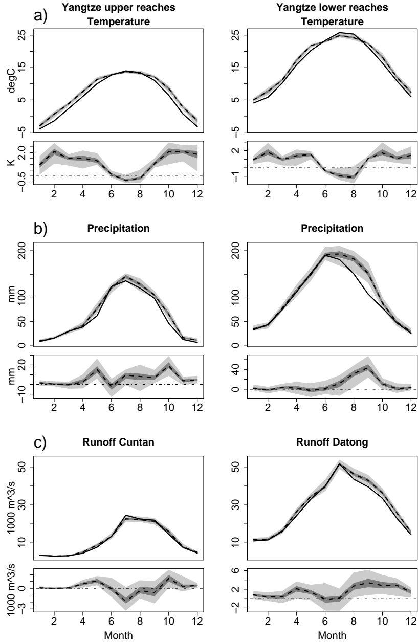
FIG. 4. Annual cycles (monthly means/sums) of a) temperature, b) precipitation and c) runoff (at Cuntan and Datong) for the upper (left) and lower (right) reaches of the Yangtze: annual cycles from the observed station data 1961 to 2000 (full line); spread (light gray shaded), inter-quartile range (dark gray shaded) and median (dashed black line) of the STAR ensemble projections (2001 to 2040). Bottom panels: Differences of future projections minus training period observations, shades and lines as in top panels.
