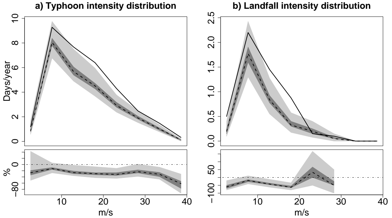
FIG. 8. a) Frequency distribution (typhoon days per year) of typhoon intensities (wind speed \text{m s}^{-1} ) in the East China Sea and b) : frequency distribution of the typhoon days with landfall. Top: Distribution from the observation period 1961 to 2000 (solid black line); spread (light gray shaded), inter-quartile range (dark gray shaded) and median (dashed black line) of the STAR ensemble projections (2001 to 2040). Bottom: Relative differences of future projections minus training period distribution.
