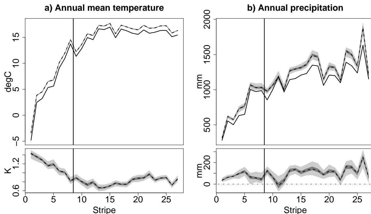
FIG. 5. Annual mean a) temperature and b) precipitation along the Yangtze: profiles from the observed station data 1961 to 2000 (solid black line); spread (light gray shaded), inter-quartile range (dark gray shaded) and median (dashed black line) of the STAR ensemble projections (2001 to 2040). Averages are taken on stripes perpendicular to the two Yangtze segments (see Fig. 3; upper and lower reaches are separated by a vertical line). The stripes are numbered along the x-axis. Bottom panel: Differences of future projections minus training period observations; shades and lines as in top panel.
