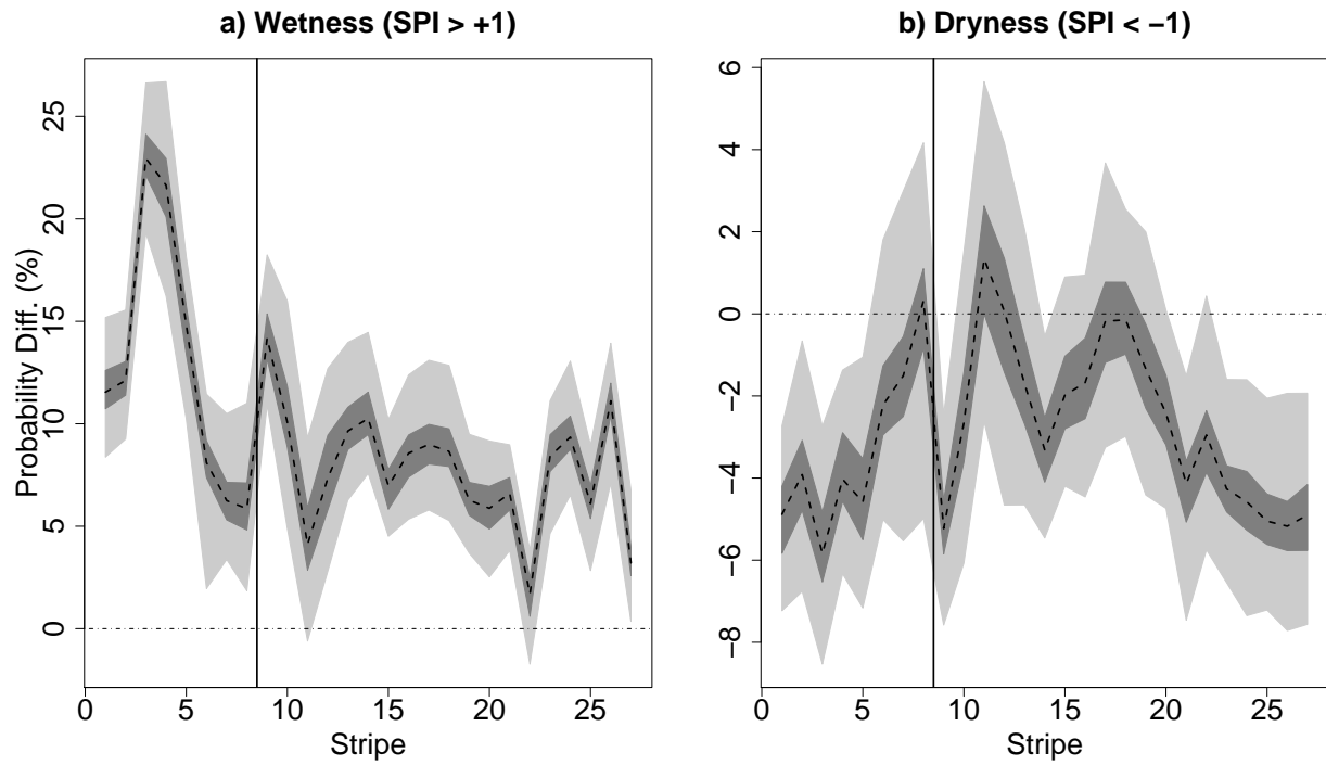
FIG. 7. Changes of a) moderate to extreme wetness and b) dryness classes of the Standardized Precipitation Index (SPI) given as differences (in percentage points) of STAR future projections (2001 to 2040) minus training period observations (1961 to 2000) along the Yangtze: spread (light gray shaded), inter-quartile range (dark gray shaded) and median (dashed black line) of projected differences. The zero-line corresponds to the probability of the training period SPI (16%).
