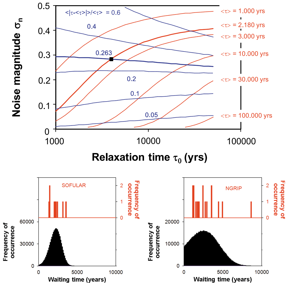
Figure 5. Parameter estimation of the process H1. (top) Isolines of constant population mean interevent waiting times \langle\tau\rangle (red) and of constant ratios between the population mean absolute deviation and the population mean interevent waiting time, \langle|\tau - \langle\tau\rangle|/\langle\tau\rangle (blue), as a function of the parameters \tau_0 and \sigma_n . Thick lines correspond to the values as obtained from the sample of 10 DO events (3–12) in the Sofular isotopic record (Table 1). The point of intersection, which is marked in black, represents our estimation of the parameters \tau_0 and \sigma_n (see text for more details). This approach yields \tau_0 \approx 4000 years and \sigma_n \approx 0.284 for the Sofular record, and \tau_0 \approx 16,000 years and \sigma_n \approx 0.355 for the NGRIP record. For each point, the length of the simulation is 10,000,000 time steps (i.e., 200,000,000 years). (bottom) The waiting time distribution as generated by the process H1 (black), using the values of the parameters \tau_0 and \sigma_n as obtained by our parameter estimation procedure. In addition to that, the histogram of the interevent waiting times as obtained from the (left) Sofular and (right) NGRIP records is also shown (red). The binning is 100 years. The ensemble size of the simulations in Figure 5 (bottom) is about 800,000 events.
