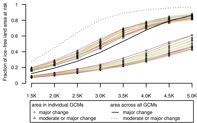
Fig. 5. Importance of climate ensemble analysis. Circles and triangles denote the area projected at risk of major or at least moderate change, respectively, by individual AOGCMs. The black solid and dashed lines mark the total area at risk across all AOGCMs. Higher total areas result from regional differences between AOGCMs.
