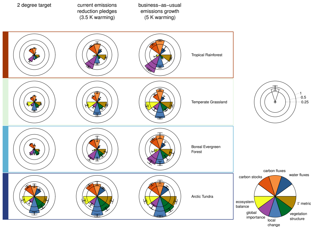
Fig. 4. Dimensions of ecosystem change for select biomes. Components of \Gamma are averaged over all grid cells belonging to the biome during the reference period. Vegetation structure: \Delta V ; local change: c \cdot S(c, \sigma_c) ; global importance: g \cdot S(g, \sigma_g) ; ecosystem balance: b \cdot S(b, \sigma_b) . Carbon stocks, fluxes and water fluxes refer to parameter subsets in Table 1. Error bars denote the range across the 19 climate patterns per GMT level. The four largest biomes (except deserts) are presented. For all 16 biome classes, see Fig. S7 in the Supplement.
