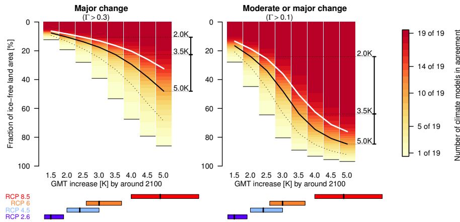
Fig. 1. Global land-surface area at risk of major ( \Gamma > 0.3 , left panel) or at least moderate ( \Gamma > 0.1 , right panel) ecosystem change by around 2100. Black and white lines denote confidence based on AOGCM agreement: solid white, high; solid black, medium; dotted black, low confidence. Range bars to the right of each panel illustrate the difference in affected area (with medium confidence) between 2, 3.5 and 5 K of warming. Coloured boxes below the main figure compare results to the 66 % range of warming expected from four Representative Concentration Pathways (RCPs) after Table 2 in Rogelj et al. (2012).
