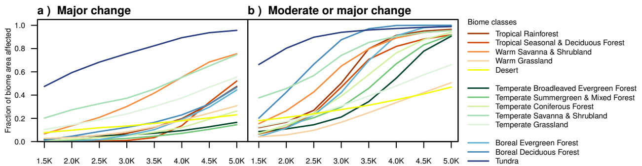
Fig. 3. Biome area affected by (a) major ( \Gamma > 0.3 ) or (b) at least moderate ( \Gamma > 0.1 ) ecosystem change by around 2100 with at least medium confidence ( \geq 10/19 AOGCMs in agreement). For other levels of confidence, see Fig. S6 in the Supplement.
