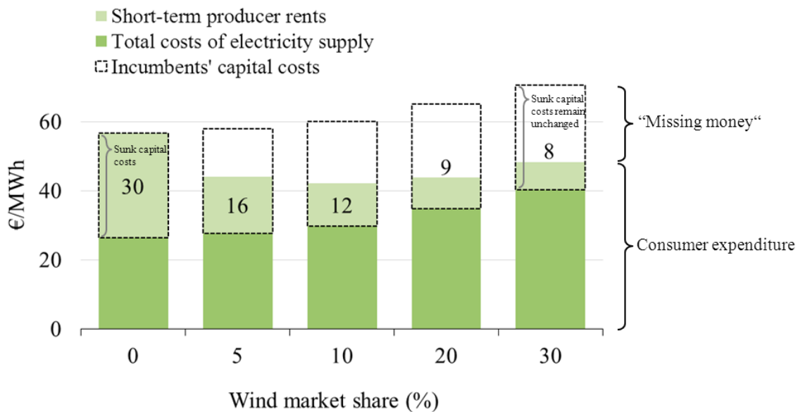
Figure 5: Rents and costs at different wind penetration rates. Numbers label short-term producer rents (light green). The sum of the colored bars is consumer expenditure. With increasing wind penetration, producer rents are transferred to consumers. At 10% wind market share, short-term consumer surplus is maximal.
