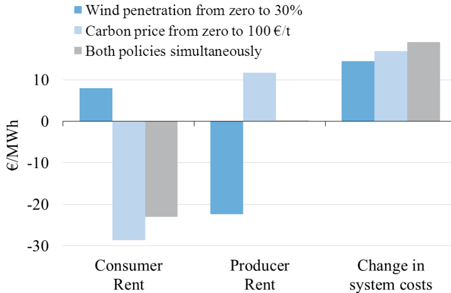
Figure 13: Change in consumer rent, producer rent, and system costs due to wind support (30%), carbon pricing (100 €/t) and a combination of the two policies. A policy mix reduced the impact on profits virtually to zero.
