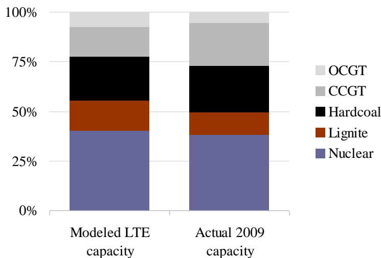
Figure 3: Model long-term equilibrium capacity mix versus historical capacity mix in 2009 for the model region. The modeled LTE capacity mix resembles quite closely to the observed data.
