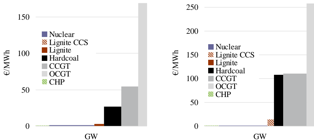
Figure 11a-b: The merit-order curve of dispatchable plants without carbon pricing (left) and at 100 €/t CO 2 . The y-axis shows bidding price that takes into account start-up costs.
