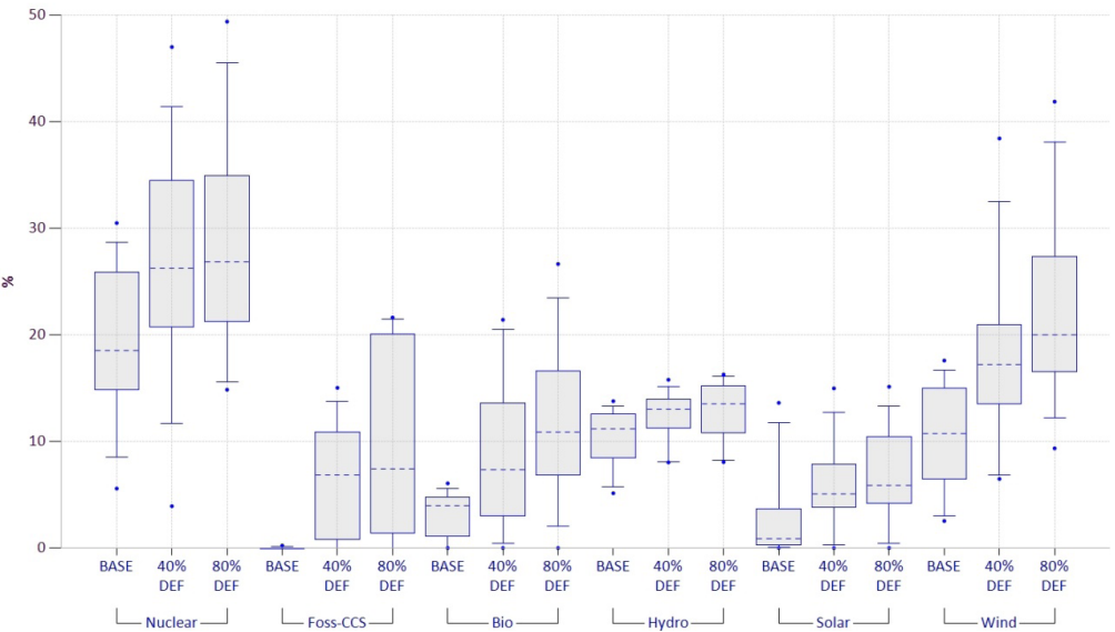
Figure 5. Percentage share of low carbon technologies in electricity mix for 2030 (upper panel) and 2050 (lower panel). The dotted line is the median, the box contains the 50% interval, the whiskers mark the 90% interval, and the dots mark the extreme values.
