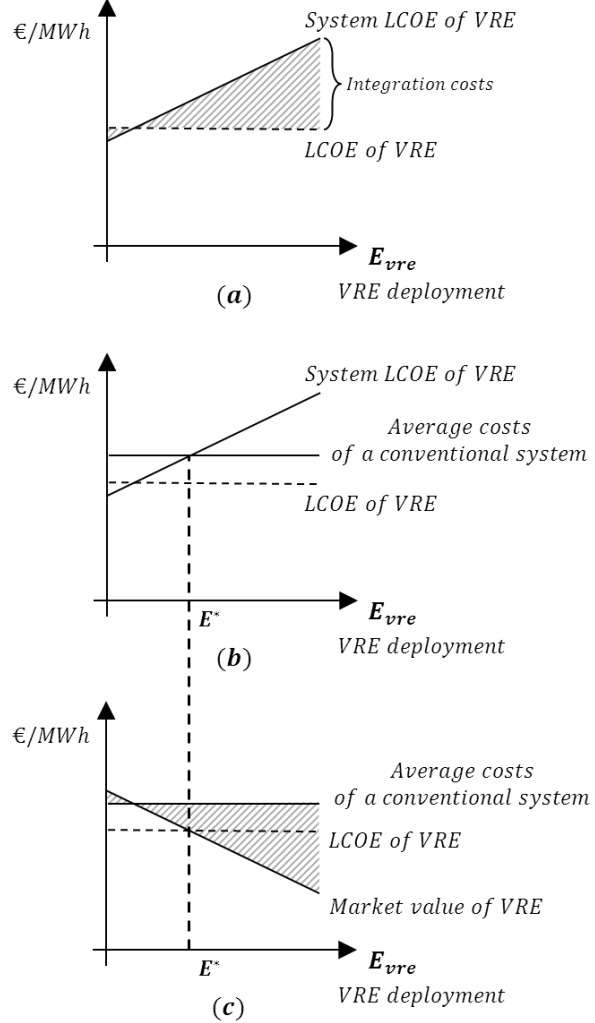
Figure 2: (a) System LCOE are the sum of LCOE and marginal integration costs (per MWh) while integration costs increase with VRE penetration. An optimal quantity E^* of VRE can be derived from (b) System LCOE or equivalently (c) the market value of VRE.
