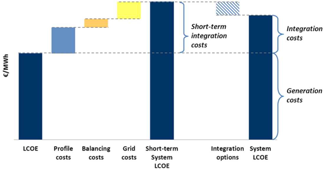
Figure 6: Integration costs are divided into three components: profile, balancing and grid costs. To some extent integration costs that occur in the short term can be reduced by integration options in the long term.
