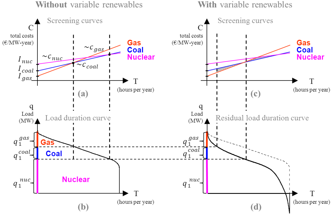
Figure 8 (illustrative): Optimal long-term capacities are derived without VRE (a, b). With VRE the LDC transforms to a RLDC (d). In the short-term perspective the capacities remain unchanged (b, d). Hence, specific costs increase because technologies operate in full-load hour ranges where they would not be cost-efficient if capacities could optimally adjust (c).
