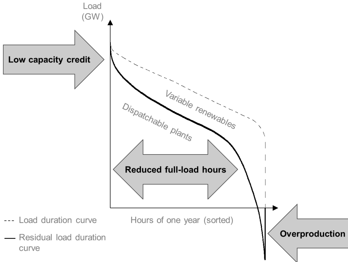
Figure 4 (illustrative): Residual load duration curves capture three main challenges of integrating VRE. While hardly any generation capacity can be replaced due to their low capacity credit, the full-load hours of conventional plants are reduced. At higher shares VRE supply exceeds load and thus cannot directly be used.
