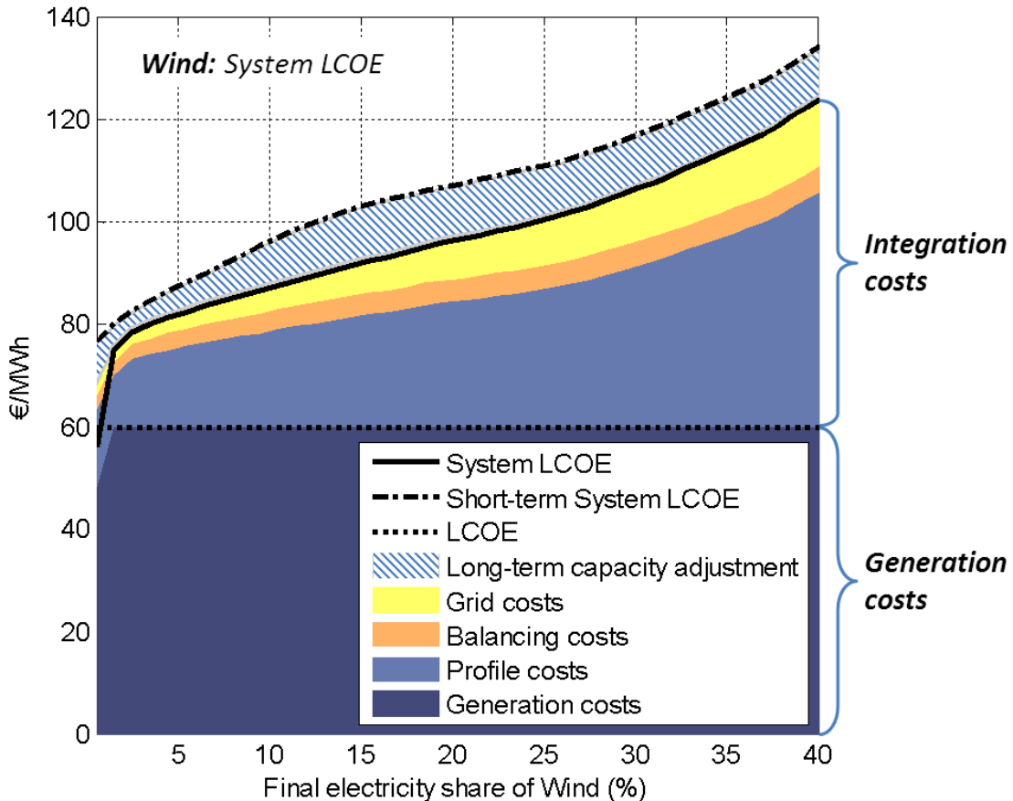
Figure 9: System LCOE for increasing shares of wind representing typical thermal power systems in Europe. Integration costs rise up to the order of magnitude of generation costs. Integration costs can thus become an economic barrier to large deployment of VRE.
