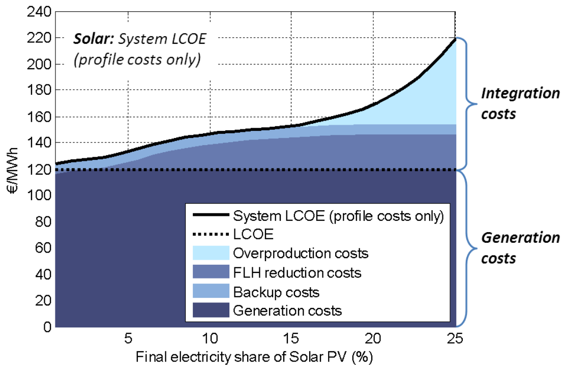
Figure 10: System LCOE (profile costs only) for increasing generation shares of wind (above) and solar PV (below) for Germany estimated with a power system model that is designed for calculating profile costs. These costs are decomposed into three cost drivers. The full-load hour (FLH) reduction of conventional plants is the largest cost driver at moderate shares, while overproduction costs significantly increase integration costs at high shares.
