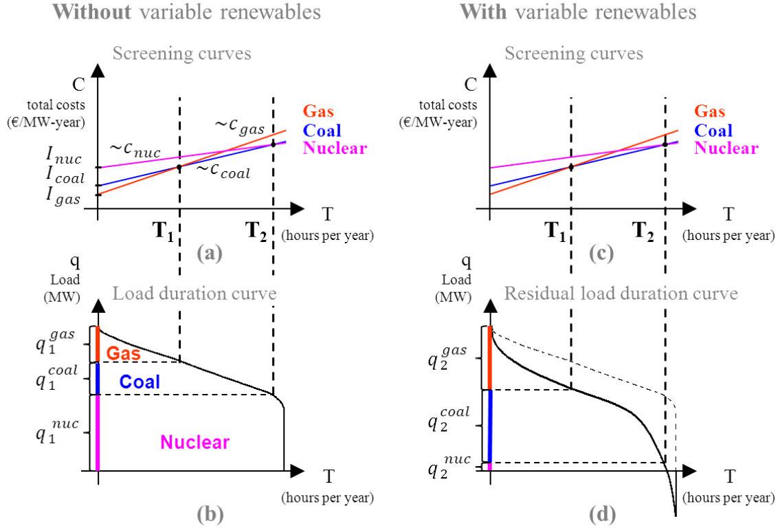
Figure 7 (illustrative): Long-term screening curves and load duration curves without (left) and with wind deployment (right). Wind changes the residual load duration curve (c, d). Thus capacities adjust towards lower fixed-to-variable-costs ratio (more gas capacity, less nuclear capacity).
