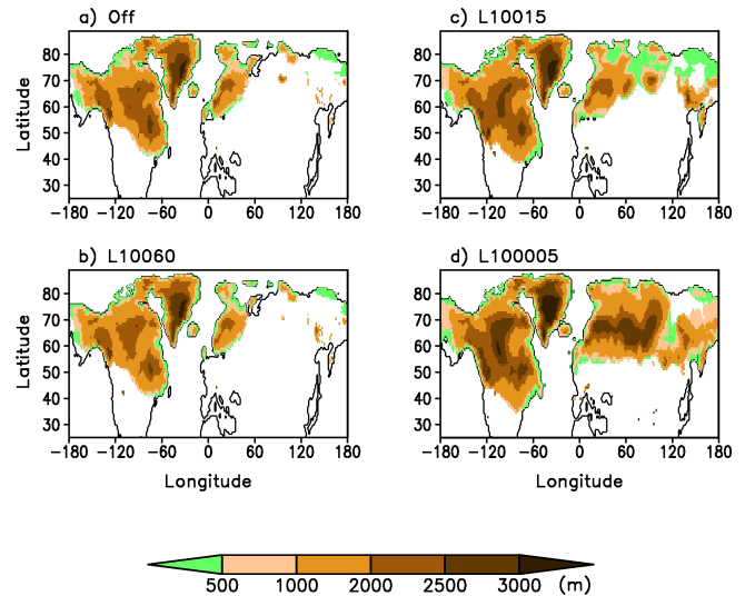
Figure 9. Simulated ice sheet extent and elevation (m) at LGM in control simulation without radiative forcing by atmospheric dust (a), and experiments using solution L1 with \text{RI} = 0.0060 (b), \text{RI} = 0.0015 (c) and \text{RI} = 0.0005 (d).
