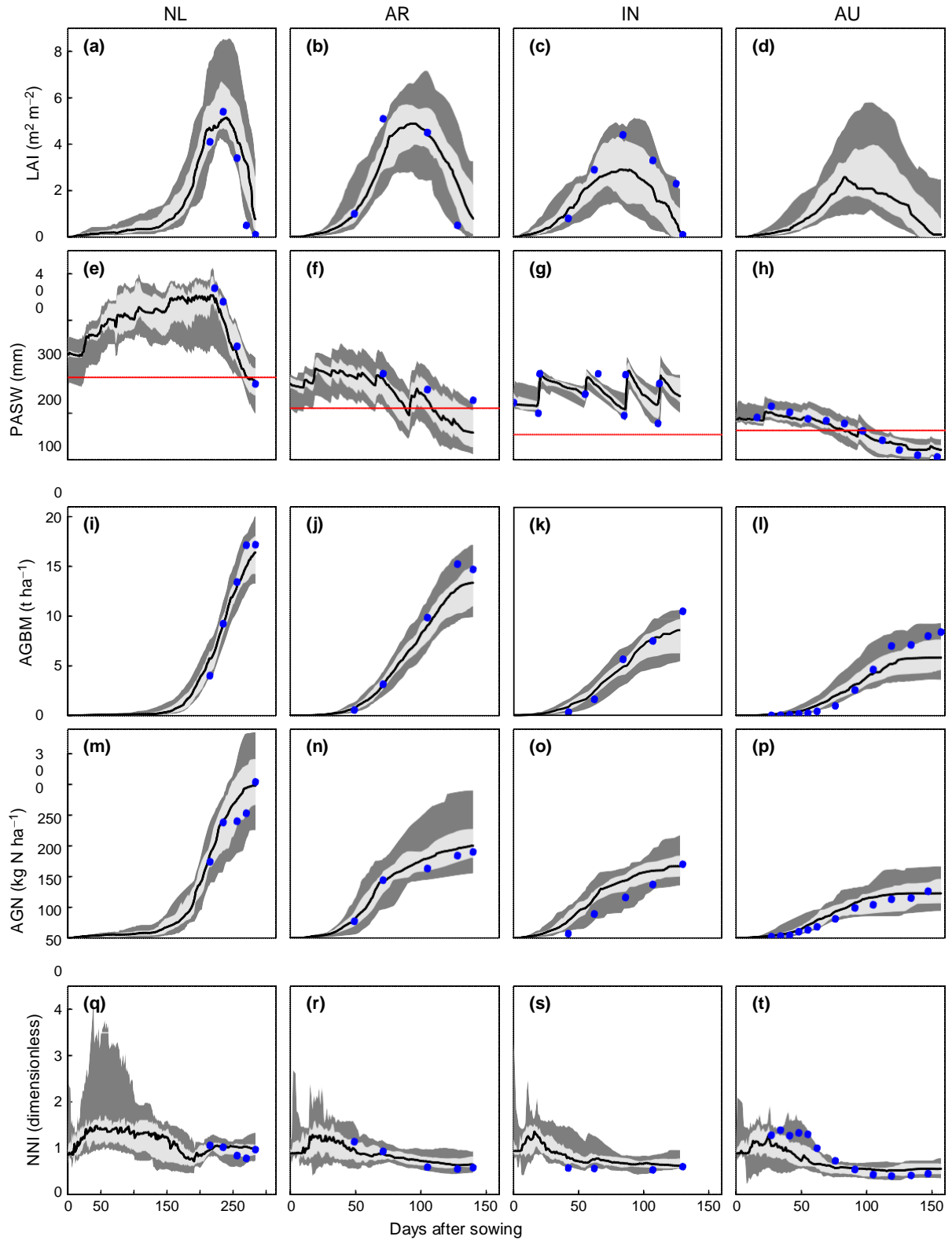
Fig. 2 Measured and simulated values of five in-season wheat crop variables for four sites. (a-d) Leaf area index (LAI), (e-h) plant-available soil water (PASW), (i-l) total aboveground biomass (AGBM), (m-p) total aboveground nitrogen (AGN), and (q-t) nitrogen nutrition index (NNI) vs. days after sowing in The Netherlands (NL), Argentina (AR), India (IN), and Australia (AU). Symbols are single measurements and solid lines are medians of the simulations (i.e. e-median). Dark gray areas indicate the 10th to 90th percentile range and light gray areas the 25th to 75th percentile range of the values generated by different wheat crop models. Twenty-seven models were used to simulate LAI and AGBM, 24 to simulate PASW, 20 to simulate AGN and NNI. In e-h the horizontal red lines indicate 50% soil water deficit.
