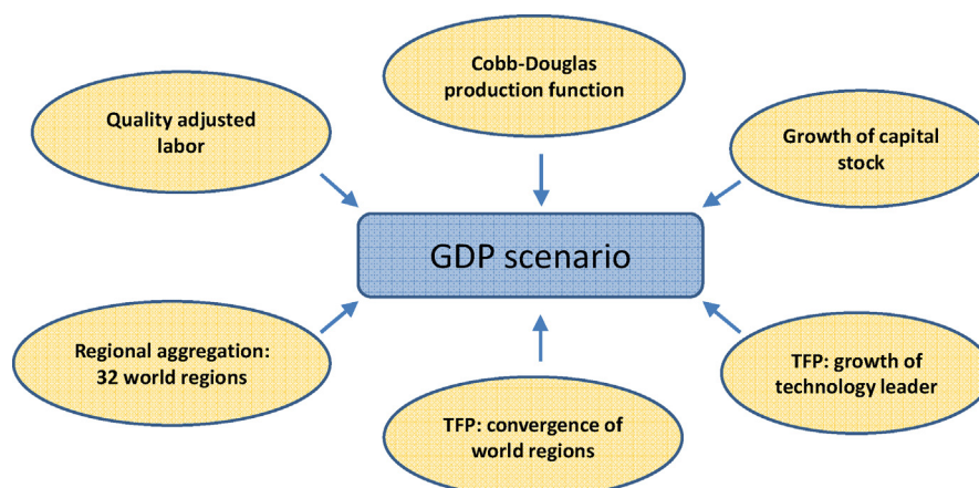
Fig. 1. Components of GDP scenario design.
