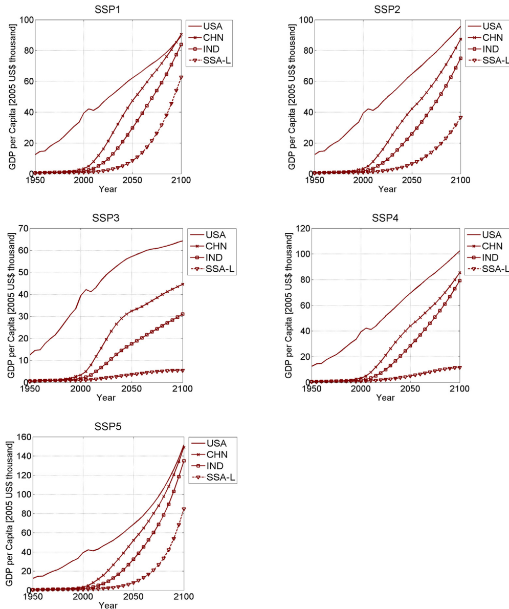
Fig. 5. Per capita income projected for USA, China, India and low income sub-Saharan Africa (each panel shows one SSP scenario).
