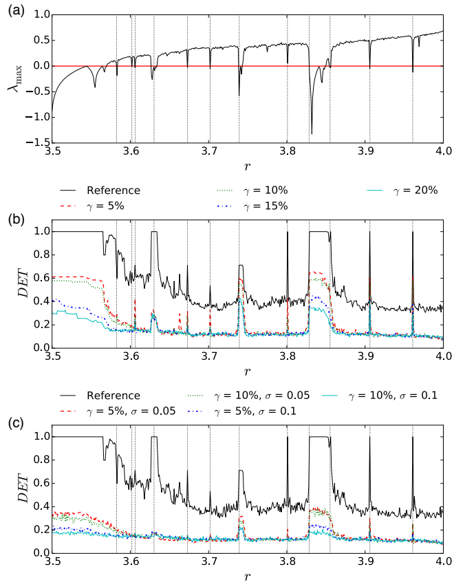
FIG. 2. (color online) RQA analyses for Logistic Map: (a) Lyapunov exponent of the Logistic Map; (b) - (c) Determinism calculated from TACTS for (b) various levels of deleting; and (c) two measurement noise levels ( \sigma = 0.05 and 0.1 ) and for two different rates of irregularity ( \gamma = 5\% and 10\% ). For details see text as well as the legends in the figures.
