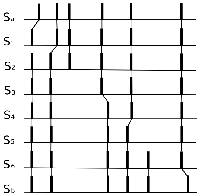
FIG. 1. Illustration of the transformation of S_a to S_b . In total S_a undergoes seven steps numbered S_1, S_2, \dots, S_6 . Note that S_7 = S_b . The path shown is a minimal-cost path and all the steps are elementary steps, like moving a spike or deleting and creating.
