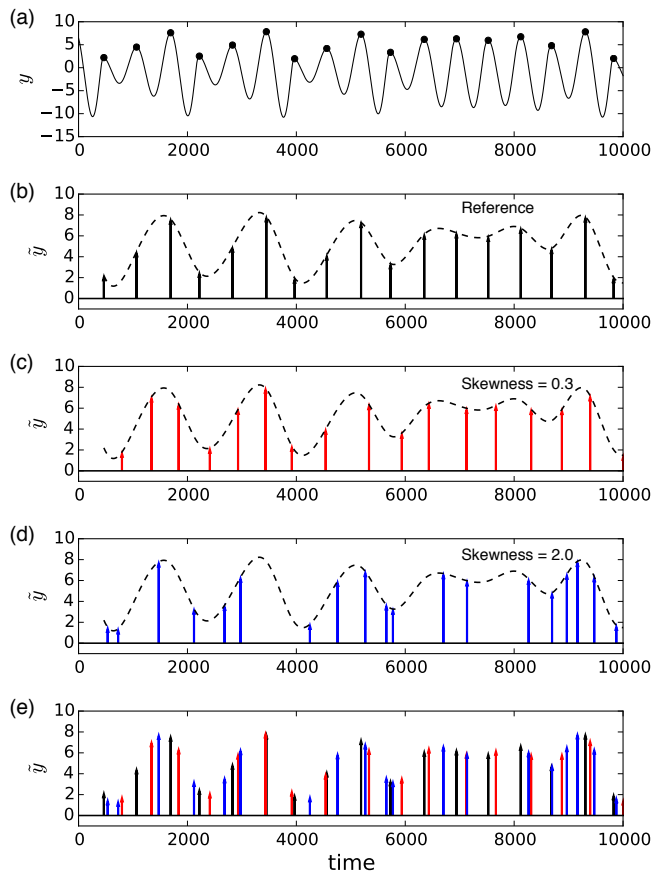
FIG. 4. (color online) The time series of Rössler: Panel (a) shows the y -component with maxima highlighted as bullets; (b) shows the result of the maximum map \tilde{Y} acting on y ; (c) shows the time series for a skewness of 0.3 and (d) for a skewness of 2.0. In panel (b) to (d) we show the interpolated time series that we draw from as a black dashed line. Panel (e) offers a comparison between the different time series and highlights their irregularity.
