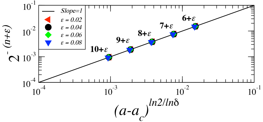
Fig. 1: While the threshold value of recurrence plot \epsilon approaches to the transition point of the logistic map a_c with (n + \epsilon, a) tuples, the scaling of the 2^{(n+\epsilon)} with (a - a_c)^{\ln 2 / \ln \delta} gives a line which has a constant slope, Slope = 1 . Also, it is shown that the scaling relation in Eq.(2) is robust for different values of \epsilon with this transformation. Numerical observations are expected in the figure, all (n + \epsilon, a) tuples with different \epsilon are on the same line with the slope equals 1 since the effective Lyapunov exponent \lambda_0 equals to \lambda 2^{(n+\epsilon)} .
