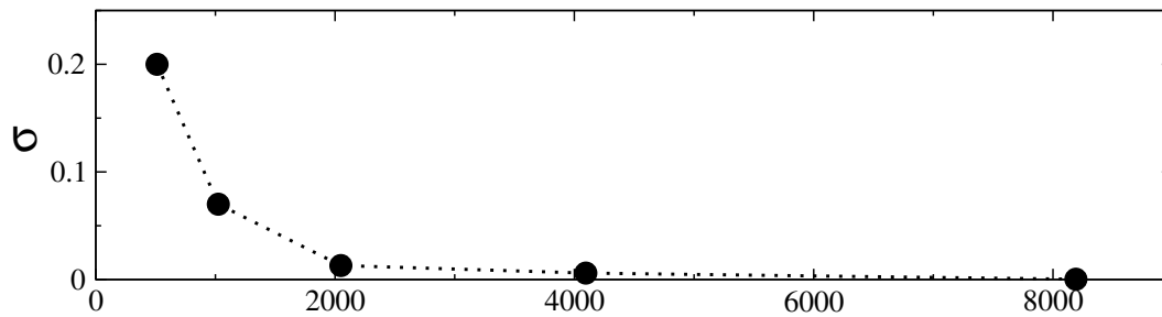
Fig. 4: The convergence behaviour of the error described by the standard deviation of the slope ( \pm\sigma ) for RR exponent \alpha while N increases.
