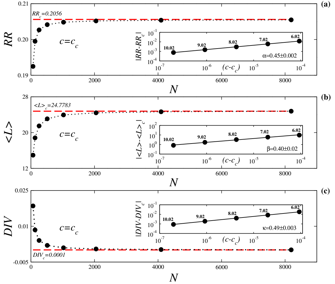
Fig. 3: The saturation and the scaling behaviours of RQA measures (a) recurrence rate RR , (b) average diagonal length \langle L \rangle and (c) just scaling of divergence DIV , for the Rössler oscillator.
