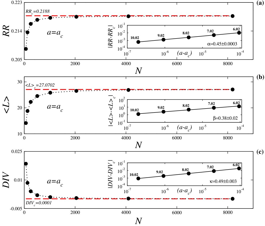
Fig. 2: The saturation and the scaling behaviours of RQA measures (a) recurrence rate RR , (b) average diagonal length \langle L \rangle and (c) just scaling of divergence DIV , for the logistic map.
