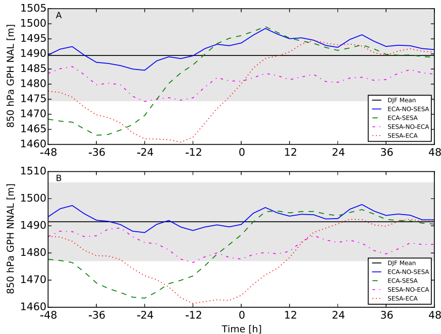
FIG. 8. (a) Mean geopotential height and standard deviations at 850 hPa over the climatological position of the NAL, represented by a box defined by 32°S, 68°W and 27°S, 65°W. Composites are shown for the four climatic regimes SESA-ECA, SESA-NO-ECA, ECA-SESA, and ECA-NO-SESA, as well as for DJF climatology. Shaded areas correspond to one standard deviation. (b) The same for the region NNAL, represented by a box defined by 25°S, 66°W and 20°S, 63°W.
