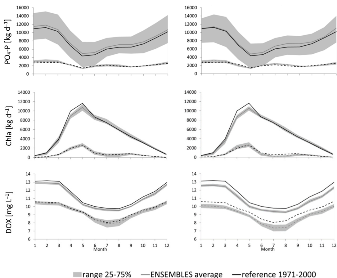
Figure 6. The long-term average monthly values of simulated discharge (Q), nutrient and chlorophyll a loads (NO 3 -N, NH 4 -N, PO 4 -P, Chla) and dissolved oxygen concentrations (DOX) with uncertainty ranges (25th/75th percentiles corresponding to 19 simulations) at the two Elbe gauges Neu Darchau (full lines) and Schöna (dashed lines) for the future periods 2021–2050 (p1, a) and 2071–2078 (p2, b) in comparison to the corresponding average values of the reference period 1971–2000 (p0).
