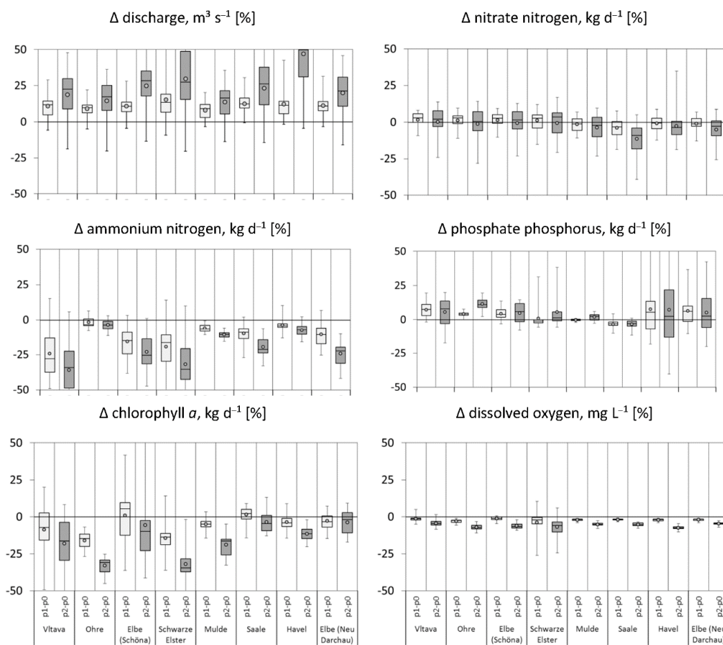
Figure 7. Ranges of the percental changes of 30-year-average river discharges, nutrients and chlorophyll a loads, as well as dissolved oxygen concentrations in the Elbe river and its main tributaries simulated with SWIM driven by 19 ENSEMBLES climate scenarios (in future periods p1 (light) and p2 (dark) compared to the reference period p0 of the same scenario). The plots visualize the following ranges: min/max (whiskers), 25th/75th percentiles (boxes), median (line) and average (dots) changes of all 19 scenarios.
