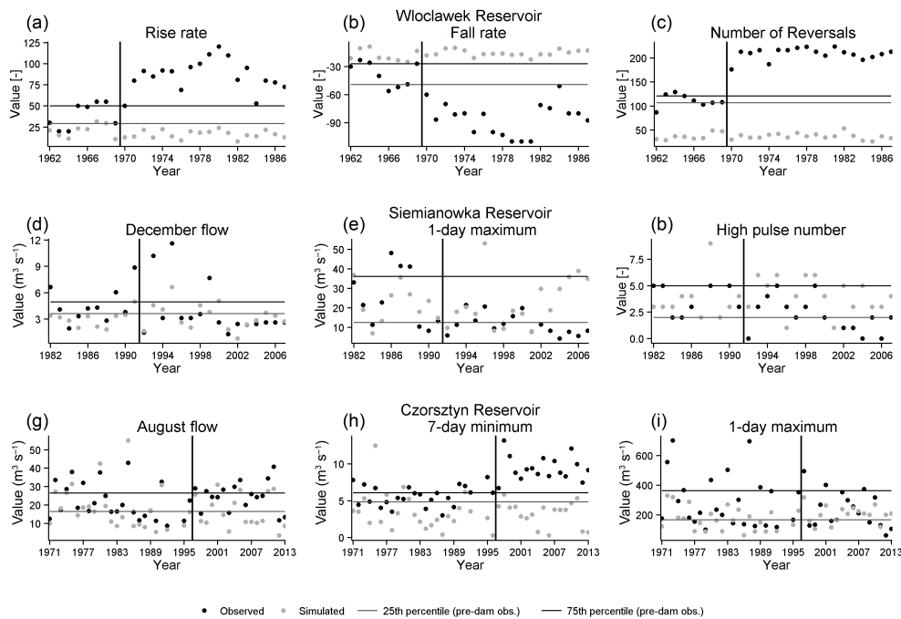
Figure 3. The effect of three dam reservoirs: Włocławek, Siemianówka and Czorsztyn on streamflow alteration assessed using observed and simulated flows. Black vertical line denotes the construction year of each reservoir. The 25th and 75th percentiles of the flow statistics were calculated based on pre-dam observed flows and delineate the likely interval of natural variability of a given statistics.
