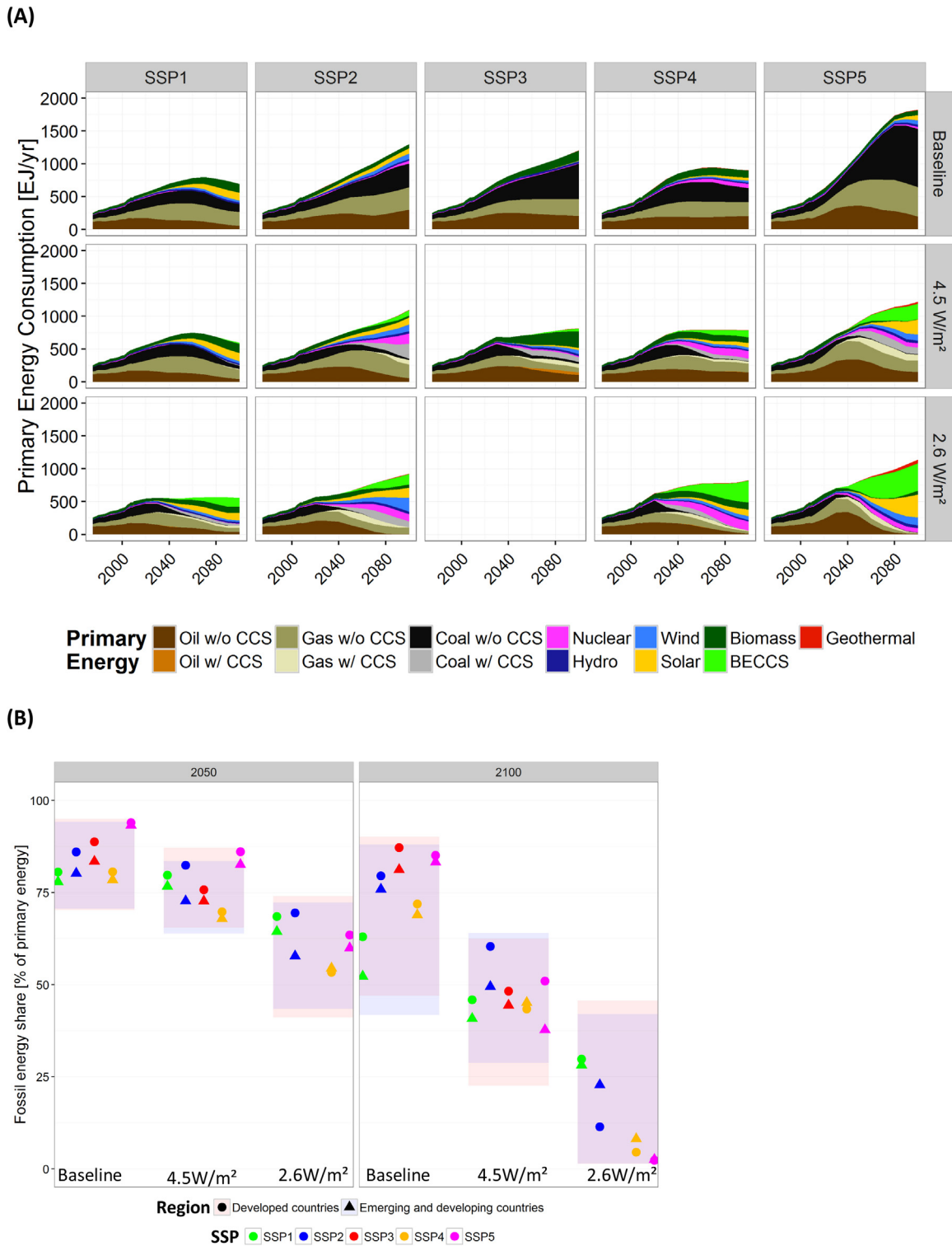
Fig. 5. Panel (A) shows global primary energy mix across SSPs and climate policy cases. Accounting for primary energy follows the direct equivalence approach. Historical data is taken from IEA (2012). Panel (B) shows the fossil fuel shares. The colored boxes indicate the ranges across all SSPs and models for the two regions.
