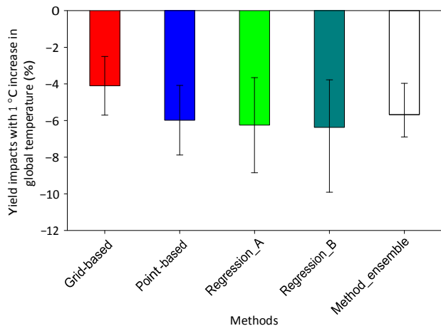
Figure 1 | Impacts of 1 °C global temperature increase on global wheat yield estimated by different assessment methods. The grid-based ( 0.5^\circ \times 0.5^\circ grid cells) method is an ensemble median from seven global gridded crop models, averaged over 30 years and aggregated over all simulated grid cells (after ref. 9). The point-based method is an ensemble median from 30 models, averaged over 30 years and aggregated over 30 global locations (after ref. 8). Regression_A is based on a country-level statistical regression from ref. 10. Regression_B is based on a global-level statistical regression from ref. 11. The error bars for the four different methods indicate the 95% confidence intervals based on multi-model ensembles in the simulations and bootstrap resampling in the statistical regressions. The mean of the method_ensemble is shown with error bars indicating the 95% confidence intervals based on medians of individual methods.
