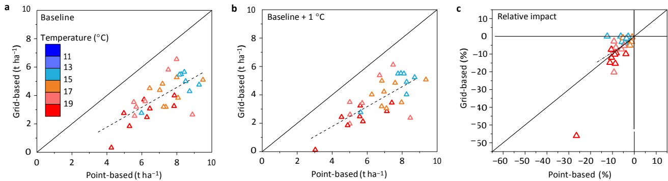
Figure 4 | Comparison of simulated multi-model median wheat yield and yield changes. a–c, Absolute wheat yields for baseline (a) and baseline +1 °C (b) periods, and relative yield change with 1 °C global temperature increase from grid-based simulations ( 0.5^\circ \times 0.5^\circ ) (from ref. 9) of cells centred around the 30 locations from the point-based study versus that from the point-based simulations (from ref. 8) (c). Note in c, the regression line is drawn without the outlier (location in Sudan). Dashed lines represent regression lines.
