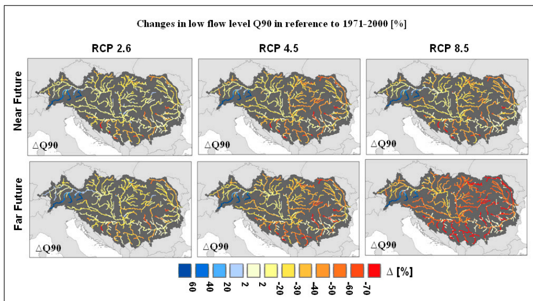
Figure 7. Projected changes in Q90 low flow magnitudes ( \Delta Q90 ) for the major rivers in the Danube basin in reference to 1971–2000 [%] for different levels of global warming (RCP 2.6, RCP 4.5 and RCP 8.5). The first row shows the relative changes up to the near future scenario period (2031–2060), and the second row up to the far future scenario period (2071–2100).
