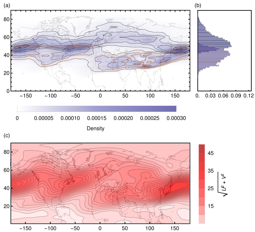
Figure 12. Probability analysis for autumn months (SON; compare with Fig. 10).
