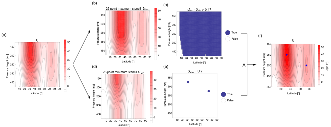
Figure 3. Rikus' scheme. In (b) the 25-point maximum stencil ( U_{\text{Max}} ) is calculated from (a) and in (d) the 25-point minimum stencil ( U_{\text{Min}} ) is calculated from (a). In (c) the condition U_{\text{Max}}(x, y) - U_{\text{Min}}(x, y) > 0.4 is examined and in (e) the condition U_{\text{Max}}(x, y) = U(x, y) . Only those points, where both conditions are fulfilled are zonal-mean jet stream cores, the blue points in (f).
