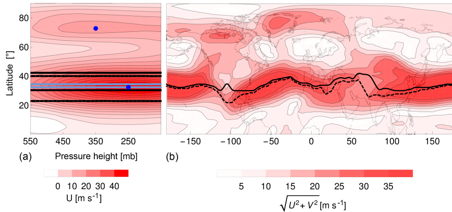
Figure 4. Panel(a): Zonal-mean latitude of the jet stream core calculated with Dijkstra’s algorithm using unoptimized weights (light-blue lines) and that computed with Rikus’ algorithm (blue circles). The black solid (dashed) lines are the borders of the PFJ (STJ) core latitude positions as calculated with Dijkstra’s algorithm. Panel(b): Polar (black) and subtropical (black dashed) jet stream cores are shown (15-day running mean around 13 January 2010).
