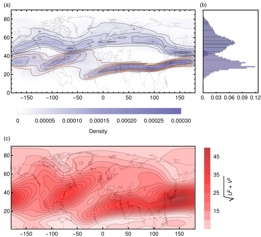
Figure 13. Probability analysis for winter months (DJF; compare with Fig. 10).
