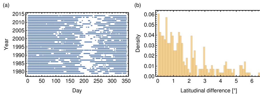
Figure 9. (a) Day–year plot for the subtropical jet stream detection scheme (compare with Fig. 8). (b) Histogram of minimum latitudinal difference between the jet stream core found with Dijkstra’s algorithm and the mean latitude from Rikus’ algorithm, in degrees, for the subtropical jet stream.
