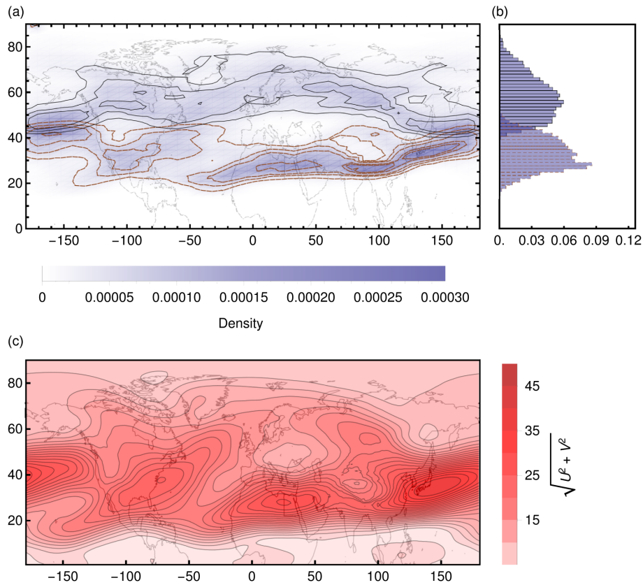
Figure 10. Probability analysis for spring months (MAM): Panel (a) and (b) show the spring probability density plot and a histogram of the jet stream occurrences (1979–2014). The brown dashed contour lines represent the subtropical jet stream, whereas the black solid contour lines represent the polar jet stream. Panel (c) depicts the climatological annual wind field (averaged over 1979–2014).
