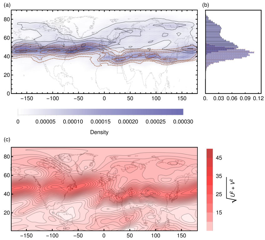
Figure 11. Probability analysis for summer months (JJA; compare with Fig. 10).
