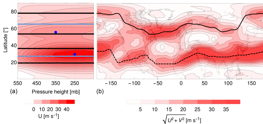
Figure 6. Fifteen-day running mean around 2 March 1979. The right panel shows three maxima (30, 50 and 75° N); because of those three maxima, the mean jet stream core found with Dijkstra’s algorithm (light-blue line) does not match with the jet stream core found by Rikus’ algorithm (blue circle).
