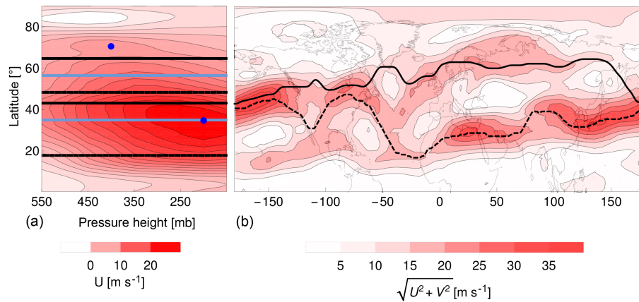
Figure 7. Fifteen-day running mean around 12 May 1979. The right panel shows only a maximum in the wind field in the region between 0 and 100° E and around 70° N latitude, which is the reason why the mean jet stream core found with Dijkstra's algorithm (light-blue line) does not match with the jet stream core found by Rikus' algorithm (blue circle).
