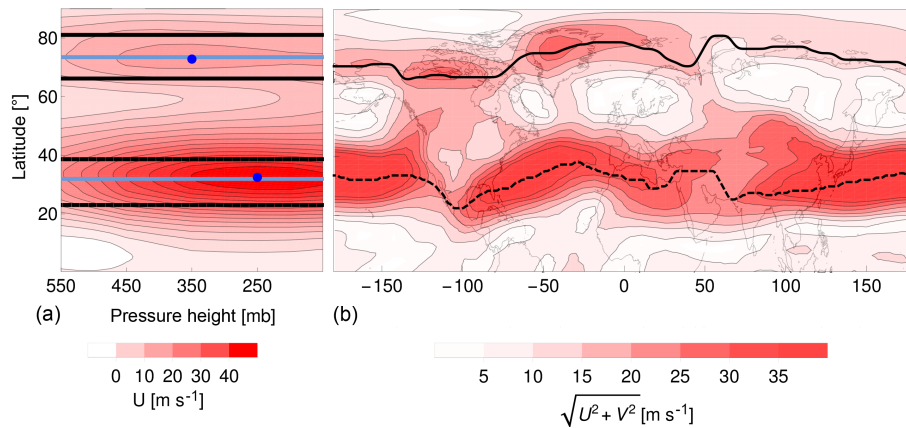
Figure 5. Fifteen-day running mean around 13 January 2010. Jet stream cores calculated with Dijkstra’s algorithm using optimized weights (compare with Fig. 2).
