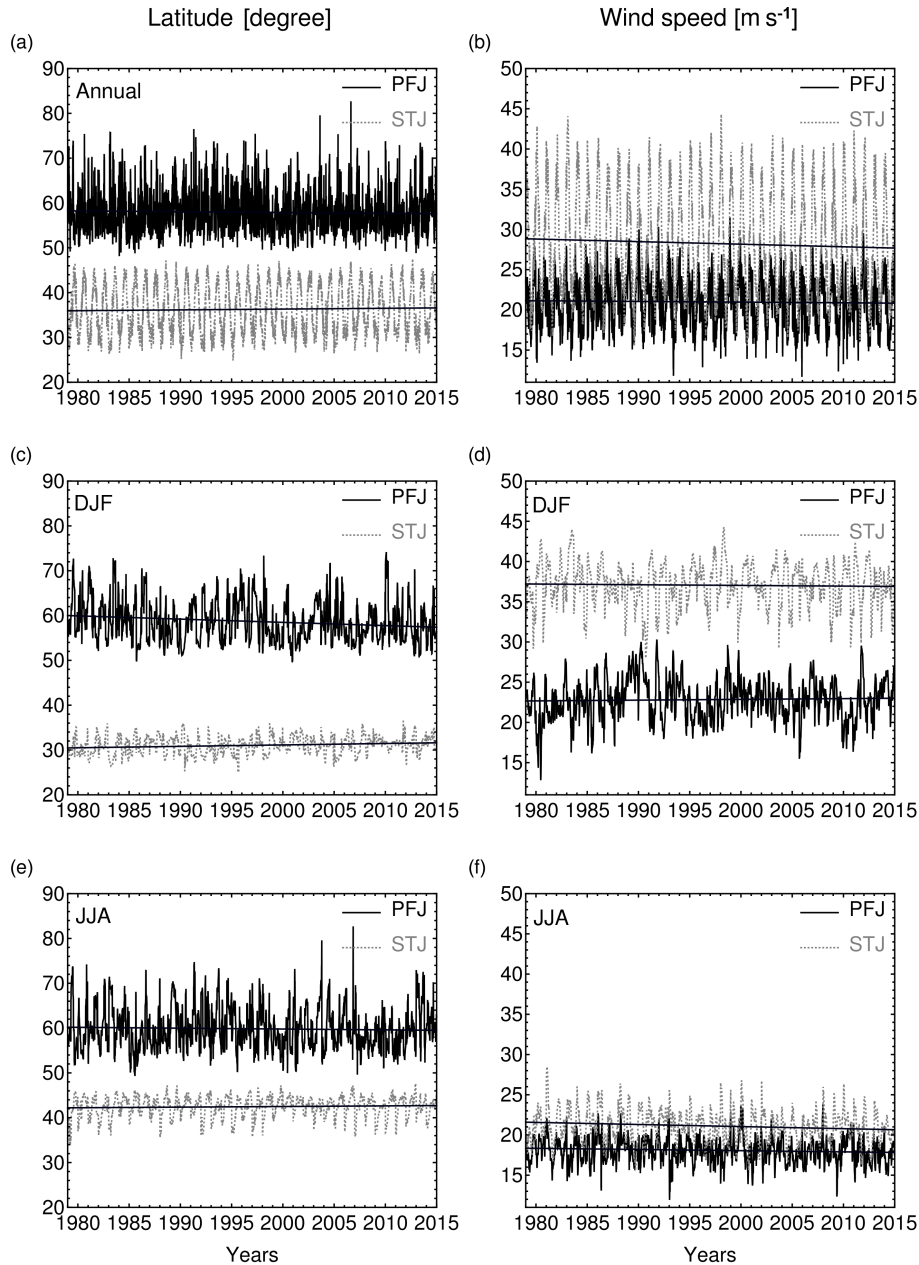
Figure 14. Annual, DJF, and JJA: mean latitudinal trends and mean wind velocity trends of the STJ and PFJ cores.
