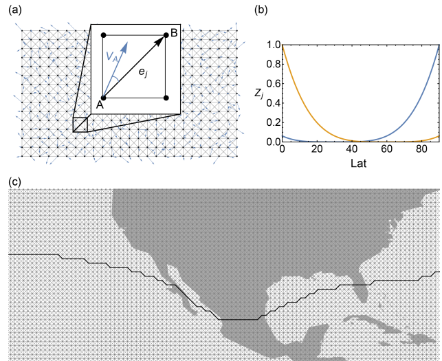
Figure 1. Definition of edge costs: (a) shows all nodes and edges as well as the wind velocities of the considered node (blue arrows) in the grid. The edge costs are computed from wind velocities (length of blue arrows, X_j ), wind direction (angle between blue arrow and black edge, Y_j ) and the latitudinal position Z_j . (b) indicates the third cost term Z_j of the STJ (blue) and PFJ (orange). The edge cost is very low in the vicinity of \phi_{\text{clim}} = 30^\circ \text{ N} for the STJ and \phi_{\text{clim}} = 60^\circ \text{ N} for the PFJ and very far away from \phi_{\text{clim}} . (c) shows the STJ (black line) in the network graph over North and Central America for a certain time period.
