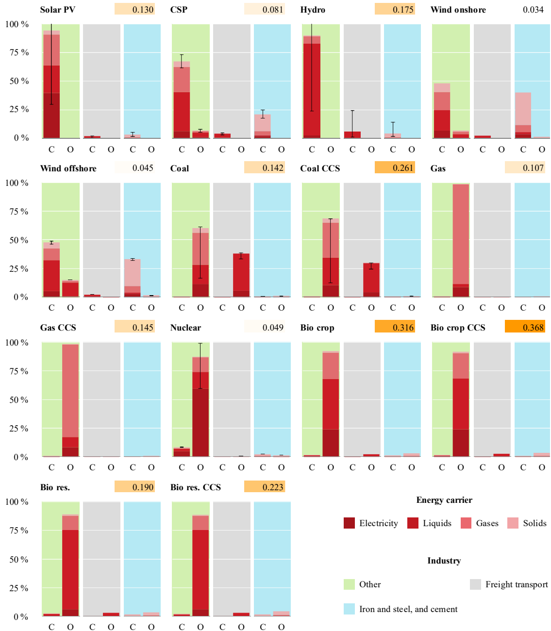
Fig. 3. Life cycle indirect energy requirements for 14 main types of power generation technologies for Europe and year 2010, broken down into phase (construction and end-of-life total, denoted by C; operational, denoted by O), energy carrier used (electricity; liquid, gaseous and solid fuels) and industry in which the use occurs (iron and steel, and cement; freight transport; other). Stacked columns represent relative contributions to total indirect energy (i.e., sum across all columns and stacked categories within columns equals 100% for each plot). For bio crop, results for a scenario assuming no restriction on types of cellulosic biomass crop available and where irrigation is allowed are shown as an example (the ‘TAX30_begr_betr_ir’ scenario’; see electronic supplement for full description). Error bars indicate extrema totals across technology subcategories relative to the mean across technology type (cf. Table 1). Vertical axes are cut at 100%, but some maxima lie above 100%: slightly >100% for solar PV, C, other; and 350% for hydro, C, other. Numerical values above plots give total indirect energy requirements in units of megajoule (MJ) energy input per MJ electricity output and exclude losses in the power production process itself. The values are shaded according to their relative magnitude (in reference to the whole set of values), with light (heavy) shading denoting small (big) magnitude. PV = photovoltaic; CSP = concentrating solar power; CCS = carbon capture and storage; Bio crop = cellulosic biomass from crops; Bio res. = biomass from forest residues.
