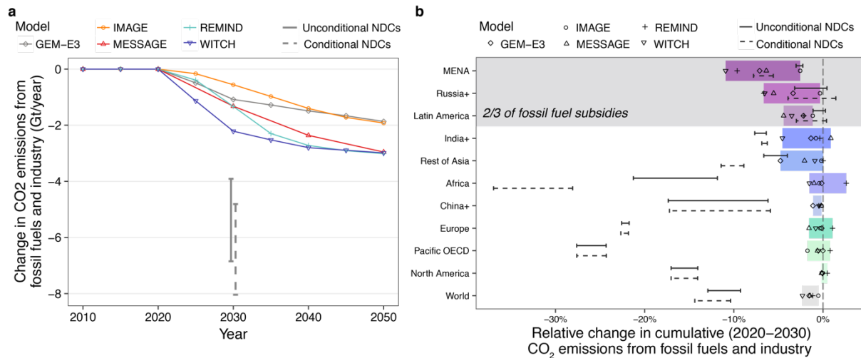
Figure 3 Global and regional impact of subsidy removal and NDCs on CO 2 emissions under low oil prices. (a) The impact of subsidy removal on global annual CO 2 emissions from fossil fuels and industry compared to each model's Baseline in Gt/year in 2020-2050. (b) Cumulative change in CO 2 emissions from fossil fuels and industry from 2020 to 2030 at the regional level from subsidy removal (colored bars – in %). In both panels, we compare the emissions impact of fossil fuel subsidy removal to the emissions impact from the NDCs under the Paris climate agreement. Unconditional NDCs are represented with solid lines and conditional NDCs with dashed lines. The NDC results are modeled using MESSAGE with the range representing different historical emissions, accounting and attribution uncertainties (see Methods, Supplementary Table 15 and ref. 21 ). See Supplementary Figure 6 for emission impacts under high oil prices, Supplementary Figure 5 for global relative changes and regional absolute changes.
