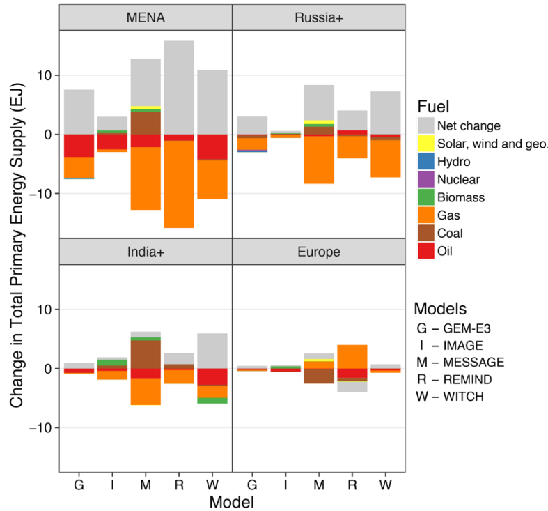
Figure 4 Change in supply of different fuels resulting from subsidy removal in 2030 in four regions. Exporting regions are represented by MENA and Russia+, developing importing countries by India+ and developed countries by Europe (see Supplementary Figure 10 for the other six regions). “Solar, wind and geo.” indicates the total change of solar, wind and geothermal power. Net change indicates a relative decrease (positive values) or increase (negative values) in the total primary energy supply. All panels depict changes under low oil prices; see Supplementary Figures 11 and 12 for energy system changes under high oil prices. Note the regional definition (Supplementary Table 9 – 14) can influence the size of energy system changes.
