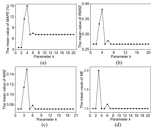
FIGURE 5. The sensitivity analysis of parameter k for NMF-AR in D_1 . The dynamic changes of four metrics of MOEs with the k eigenvectors extracted from the initial travel information matrix are plotted in (a) MAPE, (b) RMSE, (c) MAE and (d) ME, respectively. From these analyses, we find that the prediction errors are gradually stable as k is larger than 6. The same phenomenon can be observed in other datasets. Such results show that NMF-AR algorithm has a high exploration capability.
