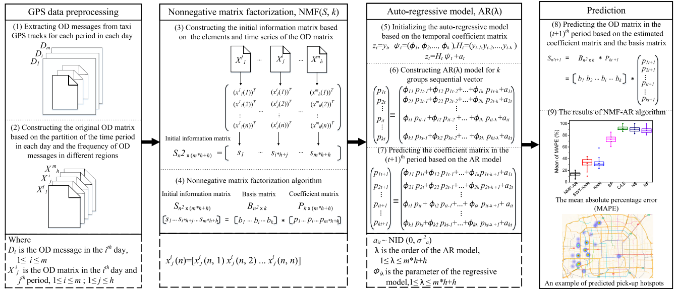
FIGURE 1. The flow chart of NMF-AR algorithm. The whole process is divided into GPS data preprocessing, nonnegative matrix factorization (i.e., NMF (S, k)), auto-regressive model (i.e., AR (λ)) and the prediction of OD matrix. As the input of NMF-AR, an OD matrix is extracted from the GPS data. The nonnegative matrix factorization (NMF) is used to reveal the pattern of OD matrix, and to extract the fundamental matrix and coefficient matrix. Based on the output of NMF, an autoregressive model (AR) is implemented to estimate the coefficient matrix in the (t + 1) th period and predict the OD matrix in the (t + 1) th period.
