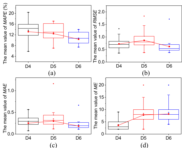
FIGURE 4. Comparisons of prediction capability of different algorithms in three spatial-based datasets. Four metrics of MOEs, i.e., MAPE, RMSE, MAE and ME are shown in (a), (b), (c) and (d), respectively. From these results, we can conclude that the computational efficiency of NMF-AR algorithm is not sensitive to the scales of the urban areas. More importantly, the NMF-AR algorithm achieves a better prediction capability with the increase of urban areas.
