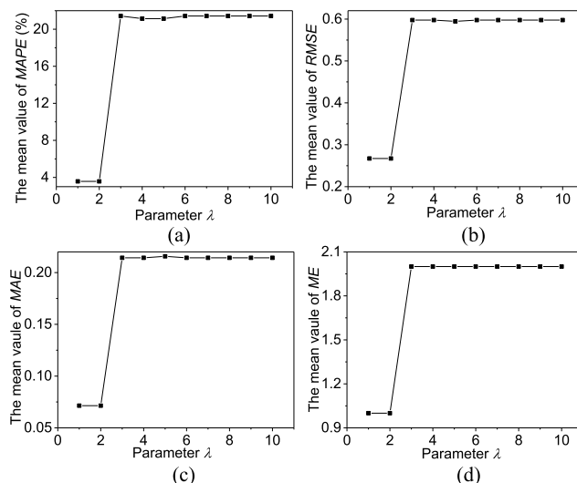
FIGURE 6. The sensitivity analysis of parameter \lambda for NMF-AR in D_1 . The dynamic changes of four metrics of MOEs with the \lambda are plotted in (a) MAPE, (b) RMSE, (c) MAE and (d) ME, respectively. The average MAPE is less than 4% if \lambda < 3 , which means that the NMF-AR algorithm achieves a high prediction capability. With the increase of \lambda , the MAPE tend to be stable around 21.23%. Results show that NMF-AR algorithm has an effective prediction capability and stability in most cases.
