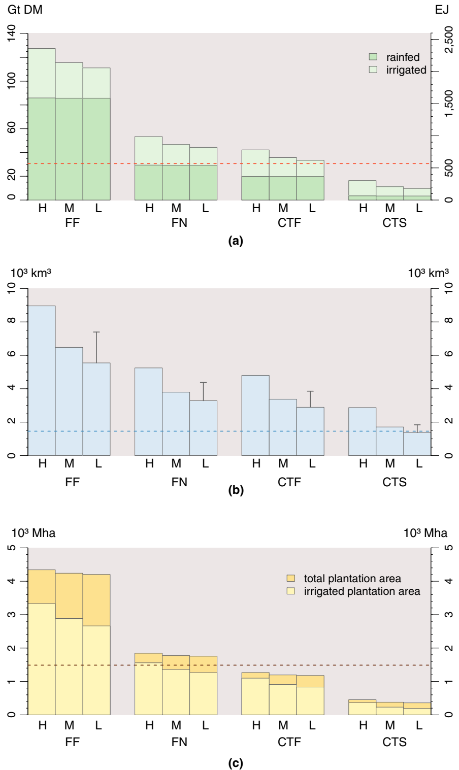
FIGURE 3 (a) Biomass supply (left: Gt DM per year, right: EJ per year) in the different scenarios and associated (b) global water consumption (10 3 km 3 ) and (c) plantation area (10 3 Mha). Land use scenarios and their abbreviation according to Table 2. The dashed orange line in (a) refers to today's total global primary energy supply according to IEA (2010). Whiskers in (b) indicate withdrawal in case of 25% conveyance losses. The dashed blue line marks current water consumption for agricultural (1,257 km 3 per year, averaged for the time period 2004–2009, according to Jägermeyr et al. (2015)) and nonagricultural (201 km 3 in year 2000) sectors, respectively. The dashed brown line in (c) marks the cropland extent around the year 2000
