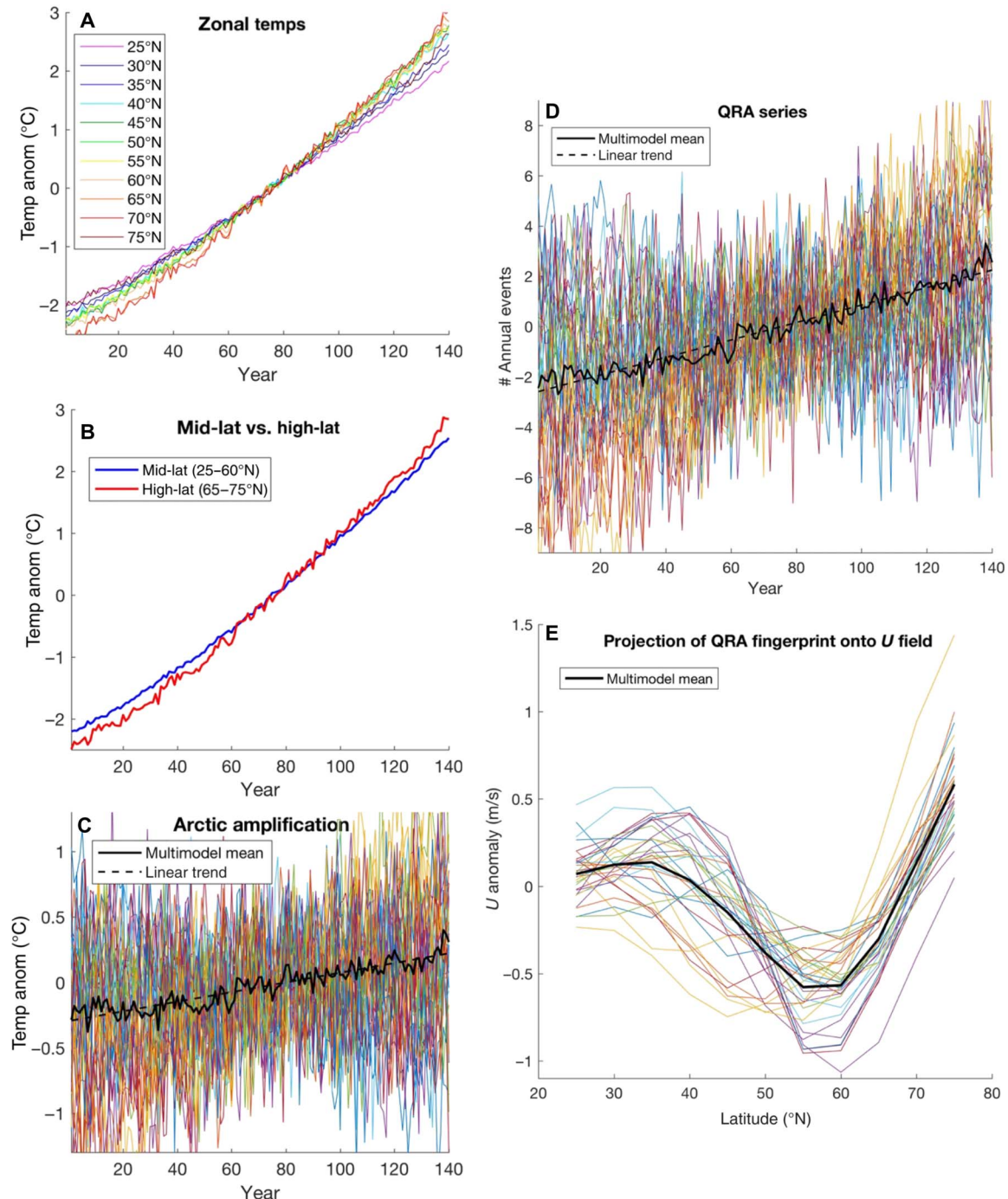
Fig. 2. Analysis of 1PCTCO 2 experiments (JJA seasonal means). (A) Time series of multimodel average zonal mean temperature anomalies. (B) Comparison of multimodel average midlatitude (25°N to 60°N) and high-latitude (65°N to 75°N) mean temperature anomalies. (C) AA index defined as high-latitude minus midlatitude series including individual simulations shown (colored curves) and multimodel mean (black solid curve), along with linear trend (black dashed lines). (D) QRA series for individual series and multimodel mean [conventions as in (C); see Materials and methods for details on scaling of QRA]. (E) Projection of the QRA fingerprint onto zonal wind anomalies.
