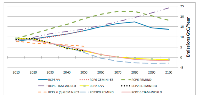
Fig. 6. Future emissions for RCP6 and RCP2.6. Source GEMINI-E3; REMIND; TIAM-WORLD; Van Vuuren et al. (2011a).
