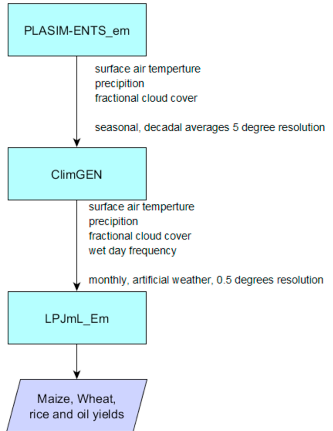
Fig. 3a. The exchange of variables between models in the bespoke framework generator (BFG2) for the PLASIM-ENTSem_ClimGEN_LPJmLem coupling. This diagram is generated automatically from the BFG2. The rectangles denote models and the parallelogram denotes outputs from the model. Arrows indicate the direction of data flow within the coupling. Model names within these figures may differ slightly from the text as they are program names.
