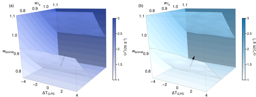
Figure 9. Strength of planetary waves \langle u^* \rangle and \langle v^* \rangle in relation to w_{T_\phi} and w_{\text{azonal}} and \Delta T_{\text{G,PD}} . The arrow points in the direction of the strongest gradient.
