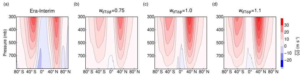
Figure 5. Zonal mean zonal wind velocity \overline{\langle u \rangle} representing the jet streams in boreal winter. Panel (a) shows ERA-Interim data, and the others show results from Aeolus with different w_{T_\phi} . In (b), w_{T_\phi} = 0.75 , in (c), w_{T_\phi} = 1.0 and in (d), w_{T_\phi} = 1.1 . All other parameters are set to standard values.
