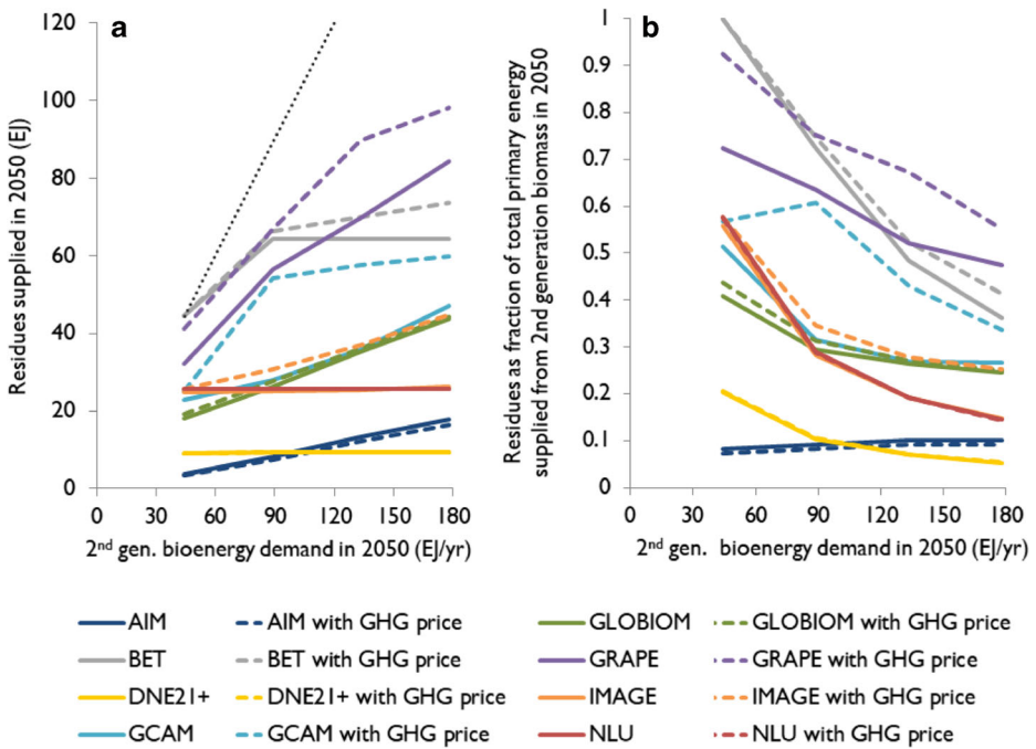
Fig. 2 Quantity of residues supplied in the studied IAMs for the year 2050, across four scenarios with increasing exogenous bioenergy demand (to 100, 200, 300, and 400 EJ/year by 2100), with and without GHG pricing (a) and residues as share of total second-generation biomass use for primary energy across the same scenarios in 2050 (b). The black dotted line indicates residues meeting 100% of exogenous bioenergy demand
