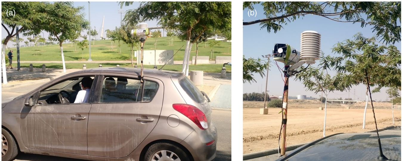
FIGURE 2 Two type T thermo-couples mounted on the rooftop of a car at about 2 m height (a) and the thermo-couples shielded in a mechanically aspirated 10 cm plastic tube (b)
