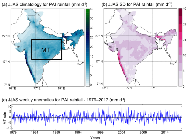
Figure 1. Rainfall climatology over India. (a) JJAS rainfall climatology over the 1979–2017 period from the Pai et al. (2015) dataset. The black box identifies the MT region. (b) Standard deviation (SD) of weekly JJAS rainfall over the 1979–2017 period from the Pai et al. (2015) dataset. (c) Time series of weekly MT JJAS rainfall over the period 1979–2017; each year contains 18 weeks, with the first week starting on 27 May.
