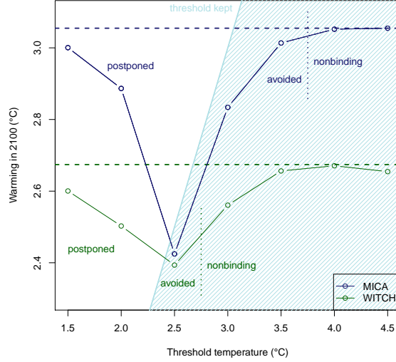
Figure 2: Temperature in 2100 reached by the grand coalition of all regions for different locations of the threshold, d = 0.04 and \sigma = 0.05
