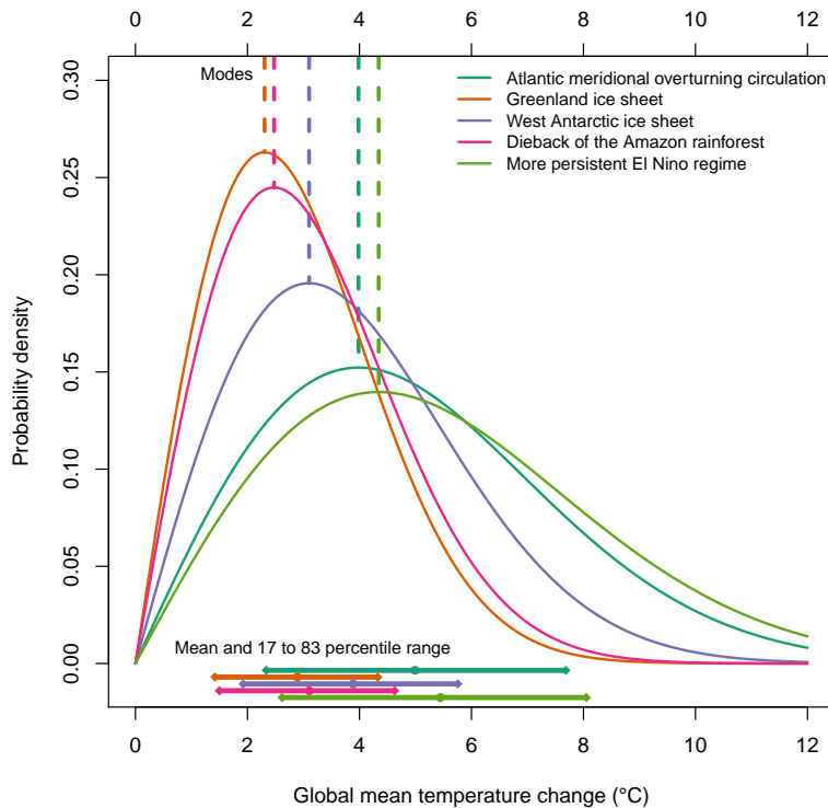
Figure S1: Different tipping points and their probabilistic temperature threshold
