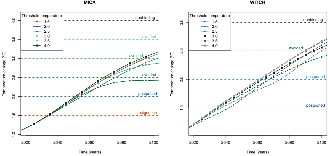
Figure 1: Temperature over time for different locations of the threshold T_s for MICA (left) and WITCH (right), d = 0.04 and \sigma = 0.05
