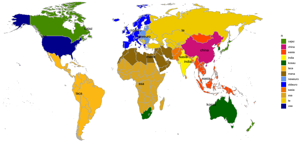
Figure S3: Regions represented as players in the WITCH model
