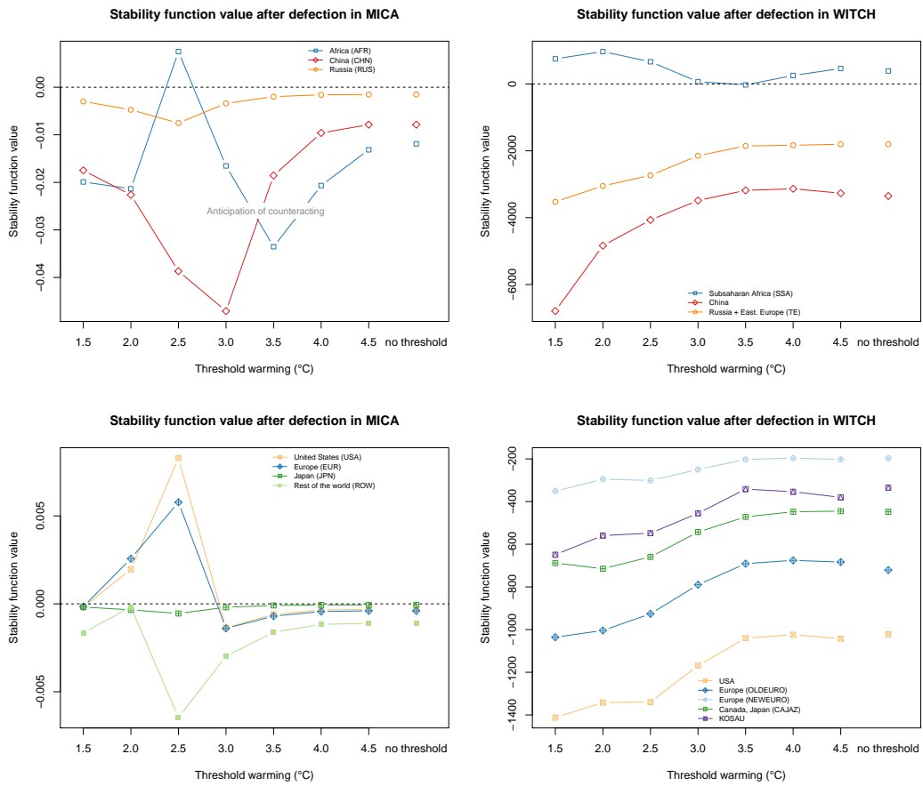
Figure 4: Stability functions for MICA and WITCH for different temperature thresholds (selected regions)
