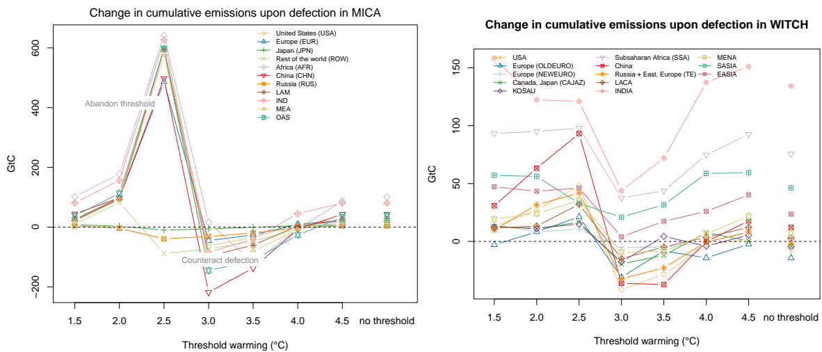
Figure S5: Changes in cumulative emissions for MICA and WITCH for different temperature thresholds
