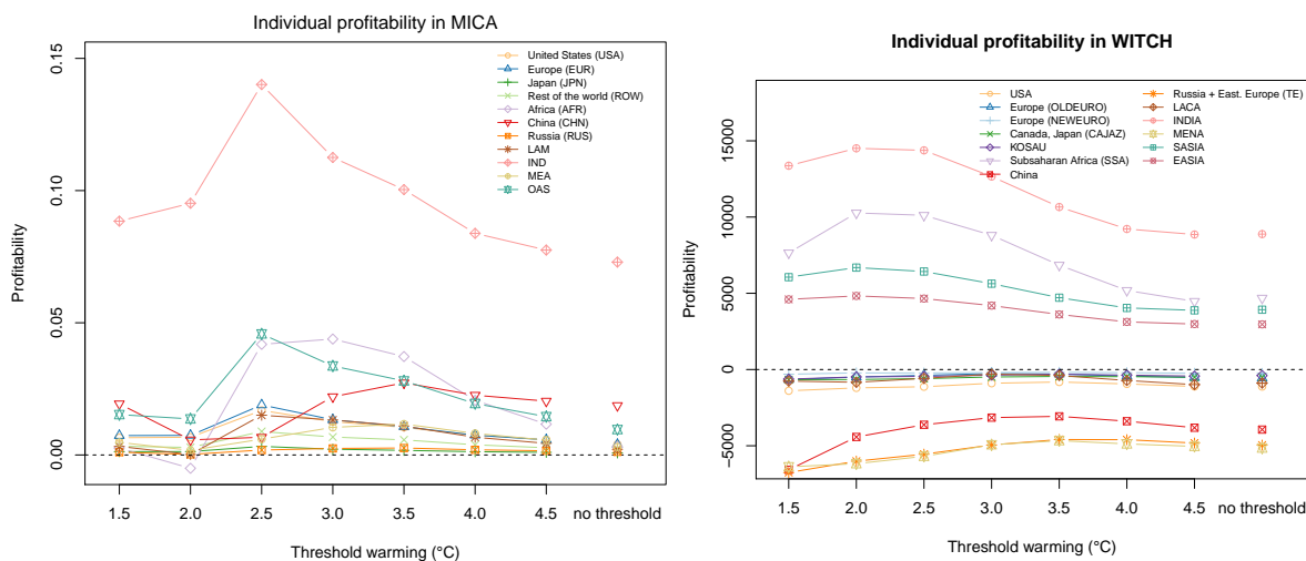
Figure S6: Profitability of the grand coalition for individual regions for MICA and WITCH at different temperature thresholds
