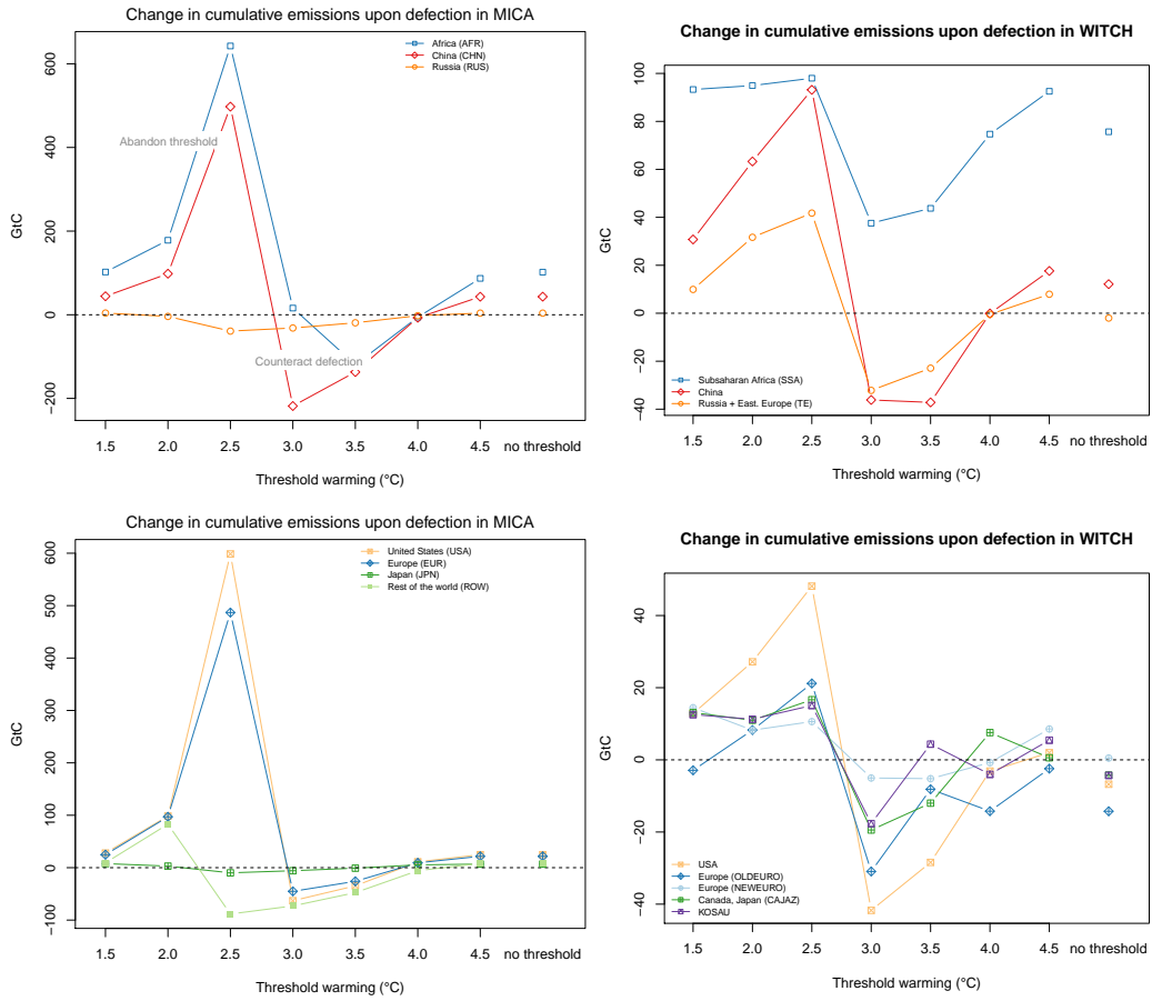
Figure 3: Changes in cumulative emissions (over the 21st century) for MICA and WITCH for different temperature thresholds (selected regions)
