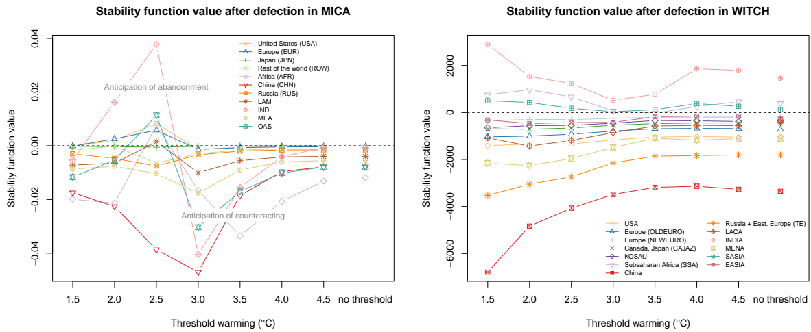
Figure S4: Stability functions for MICA and WITCH for different temperature thresholds
