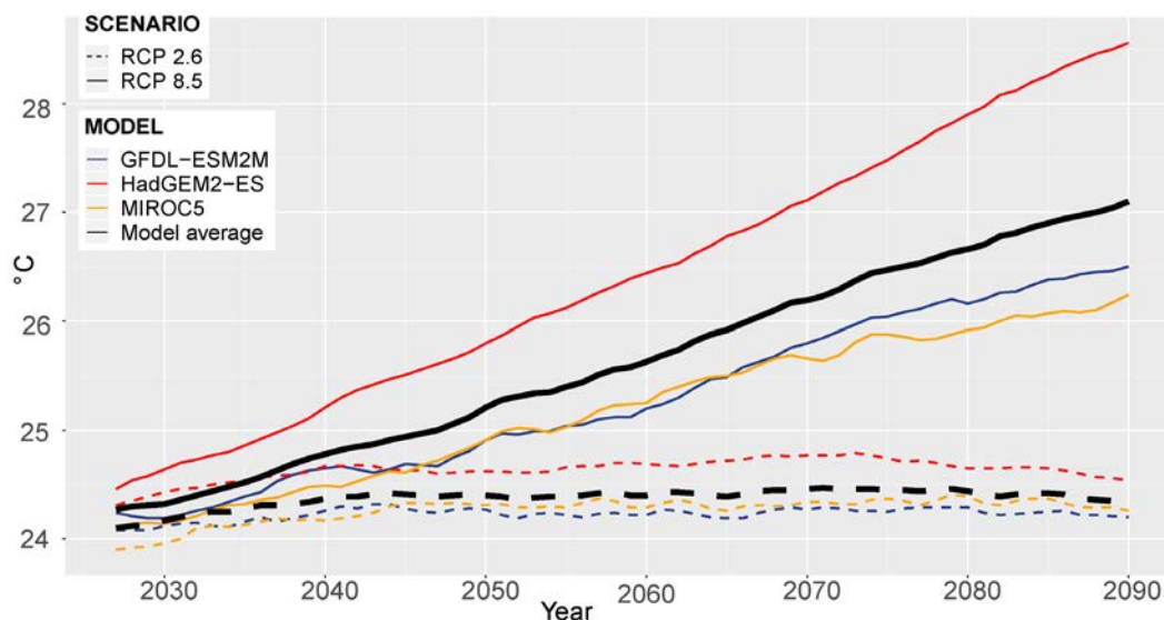
Figure 6: Projected mean annual temperature over Ethiopia for two scenarios and three climate models. The graph shows the 20-year moving average.
