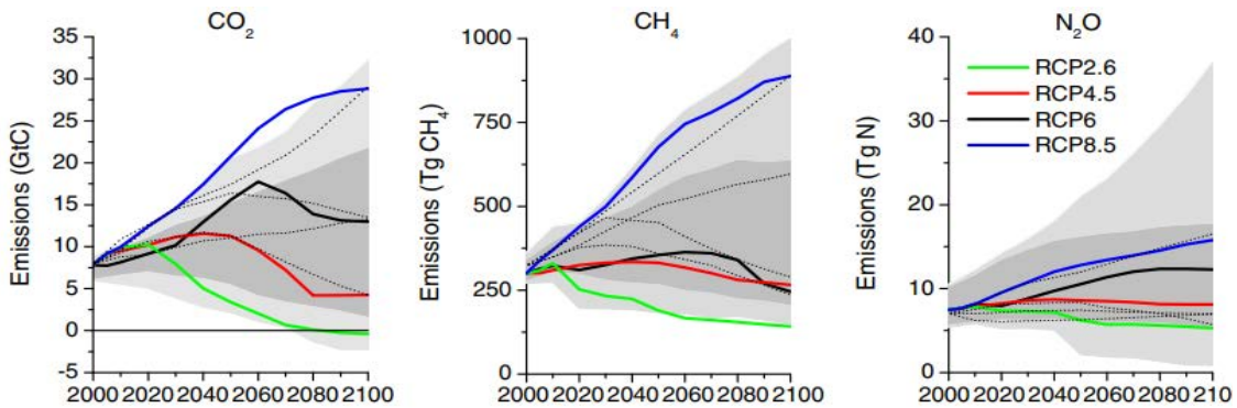
Figure 2: Emissions of main greenhouse gases across the RCPs. Grey area indicates the 98 th and 98 th percentile (van Vuuren et al., 2011).
