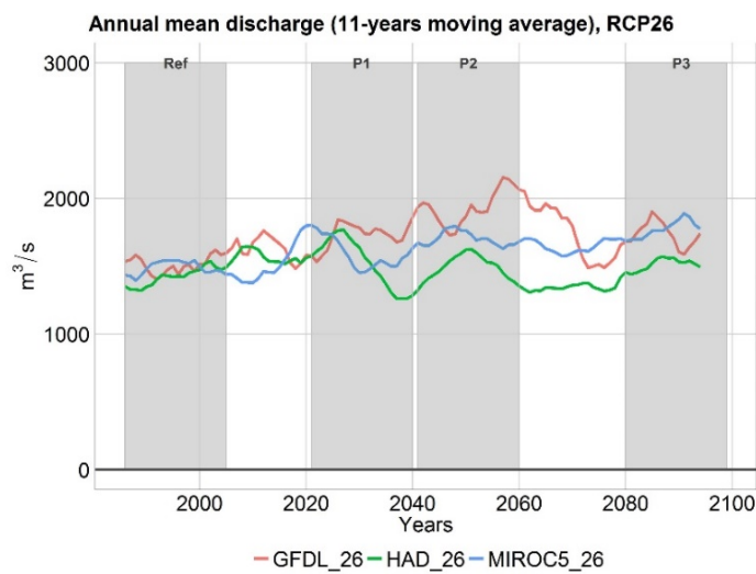
Figure 14: Annual mean discharge at the Sudan border gauge (11-years moving average) under RCP2.6.
