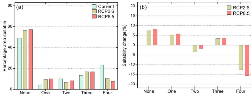
Figure 28: Suitability of multiple crops in Ethiopia under current and projected climatic conditions.
