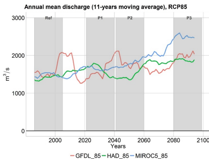
Figure 15: Annual mean discharge at the Sudan border gauge (11-years moving average) under RCP8.5.
