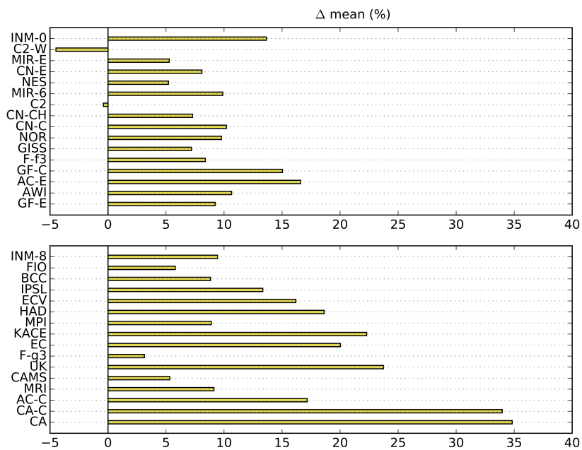
Figure B1. As in Fig. but for SSP2-4.5. The mean over all models is +11.9%
