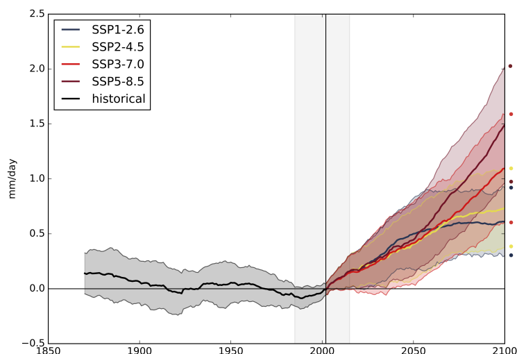
Figure 5. Multi-model mean of Indian summer monsoon rainfall (mm/day) over displayed area in Fig. 3 for 1870-2100 relative to the mean (horizontal black line) in 1985-2015 (grey background) for the four scenarios SSP1-2.6, SSP2-4.5, SSP3-7.0 and SSP5-8.5. The 20 years backwards smoothed time series of one ensemble member per model was used to calculate the multi-model mean. Shading in the time series represents the range of mean plus/minus one standard deviation marked with circles on the right side of the Figure. Availability of the models according to Table 1.
