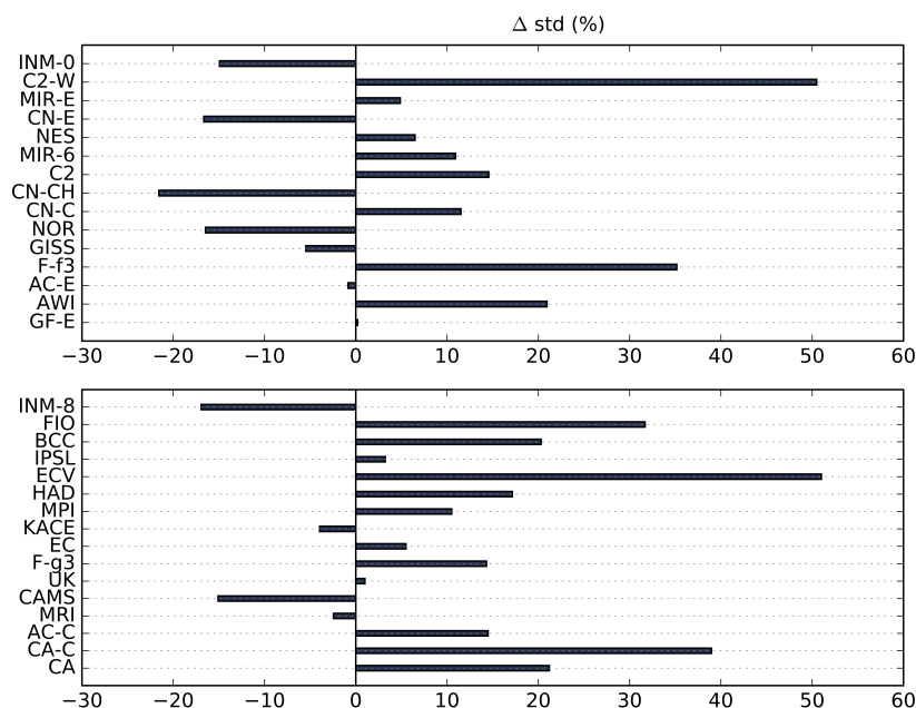
Figure G1. As in Fig. but for SSP1-2.6.
