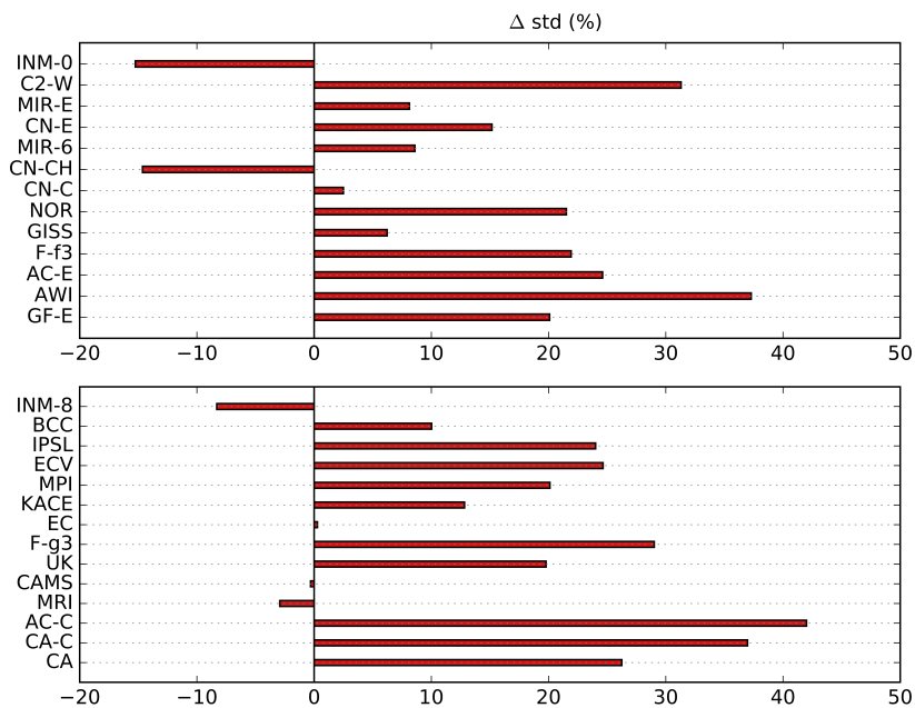
Figure E1. As in Fig. but for SSP3-7.0.
