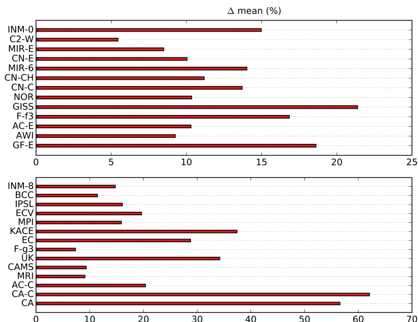
Figure A1. As in Fig. but for SSP3-7.0. The mean over all models is +18.6%. Please notice the different scales in the lower panel.
