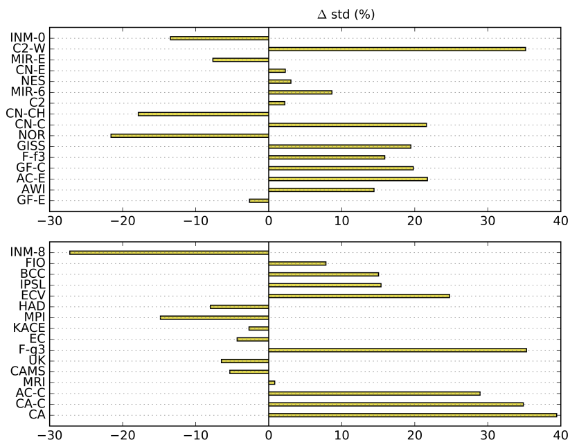
Figure F1. As in Fig. but for SSP2-4.5.
