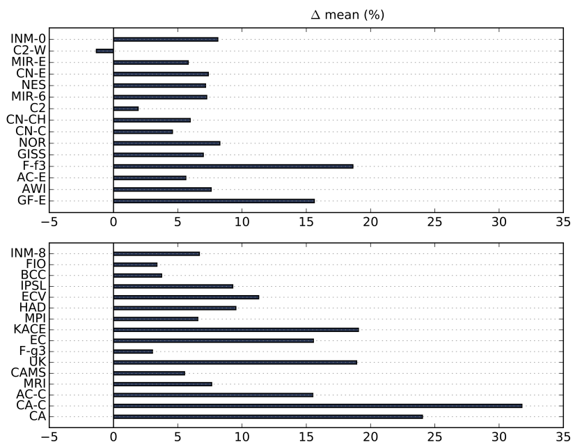
Figure C1. As in Fig. but for SSP1-2.6. The mean over all models is +9.7%
