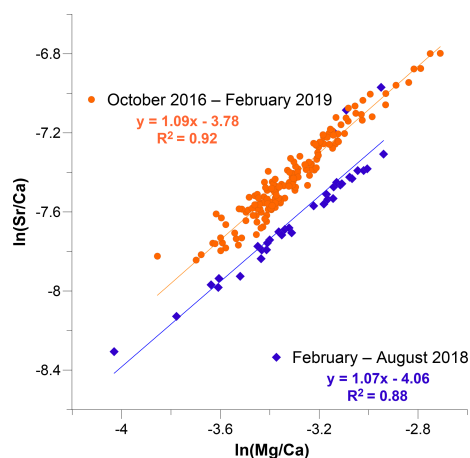
Figure 15. Drip water \ln(\text{Mg}/\text{Ca}) versus \ln(\text{Sr}/\text{Ca}) ratios in Waipuna Cave. Blue diamonds indicate samples collected between late February to the end of August 2018; orange circles are for all other samples collected between October 2016 and February 2019.
