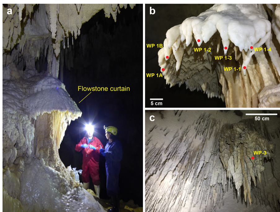
Figure 2. (a) Flowstone formation in the Organ Loft chamber (Photograph courtesy of Inken Heidke). (b) Drip sites at the flowstone curtain. (c) Stalactite cluster where drip site WP-3 is located, hanging from the ceiling 6 m high in an inclined plane.
