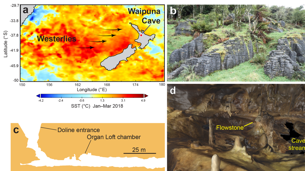
Figure 1. (a) Geographical location of Waipuna Cave and its climatic settings during La Niña conditions in summer 2018, with the direction of the Westerlies. Source data: OSTIA. SST: sea surface temperature. (b) Pancake limestone outcrop landscape above Waipuna Cave. (c) Cross section through the entrance and first stretch of Waipuna Cave. (d) 3D model of the “Organ Loft” chamber photo taken by John Hellstrom using structure-from-motion (SfM) mapping.
