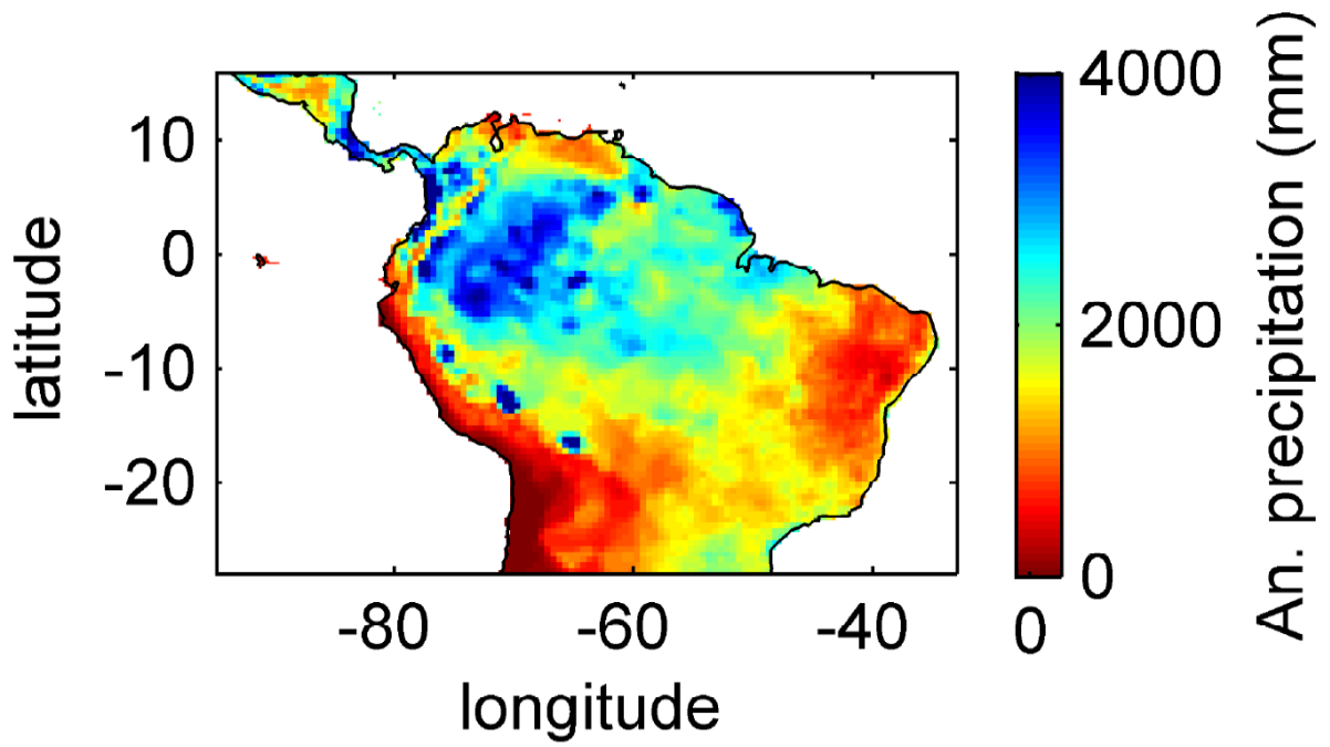
Figure S1: Mean annual precipitation for 2001-2010 under CRU climate input.
