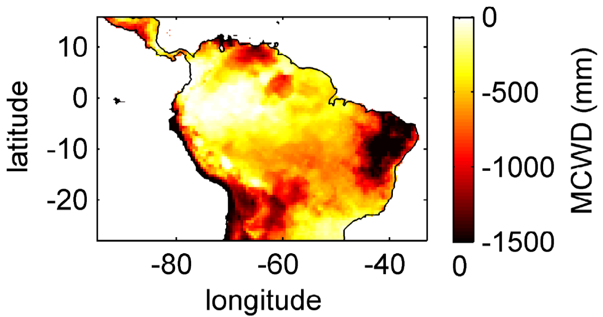
Figure S2: Mean annual MCWD for 2001-2010 under CRU climate input.
