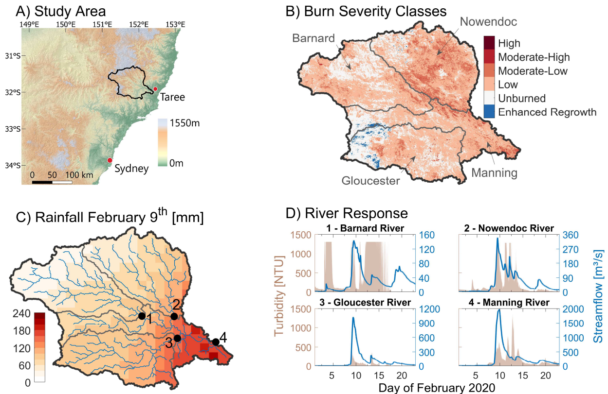
Figure 2: Study area. A) The Manning River catchment is located 250 km north of Sydney in one of the steepest regions of New South Wales, Australia. B) Fires affected the tributaries of the Manning River differently, with the highest burn severities occurring in the Nowendoc catchment. C) Gridded rainfall data for February 9 th , 2020, show increasing rainfall totals towards the coast. 1-Barnard River (Mackay), 2-Nowendoc River (Rock’s Crossing), 3-Gloucester River (Doon Ayre), 4-Manning River (Killawarra). D) Turbidity in brown and discharge in blue for Manning River and its tributaries between February 1 st and 22 nd .
