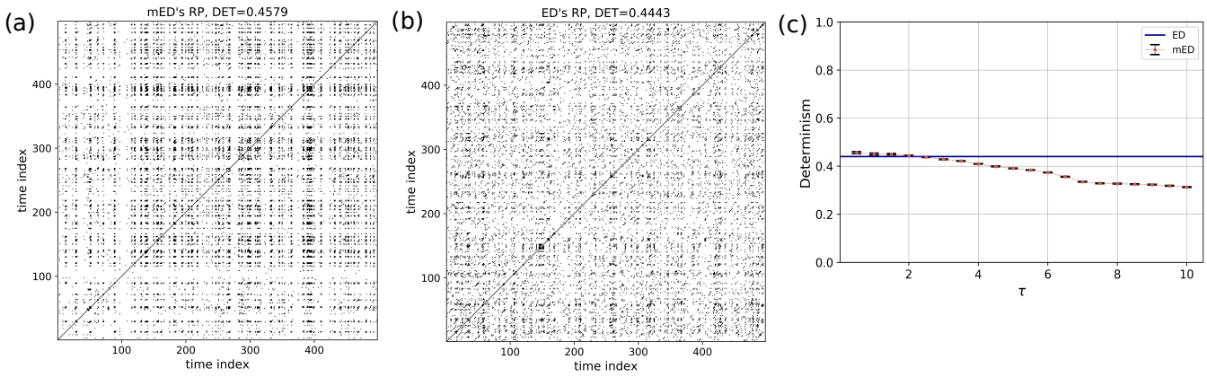
Figure 8. RP of a homogeneous Poisson process (Fig. 7a) using (a) mED, (b) ED; (c) comparison of DET for 300 realisations using ED (blue horizontal line) and using mED for varying \tau in range 0 to 10.
