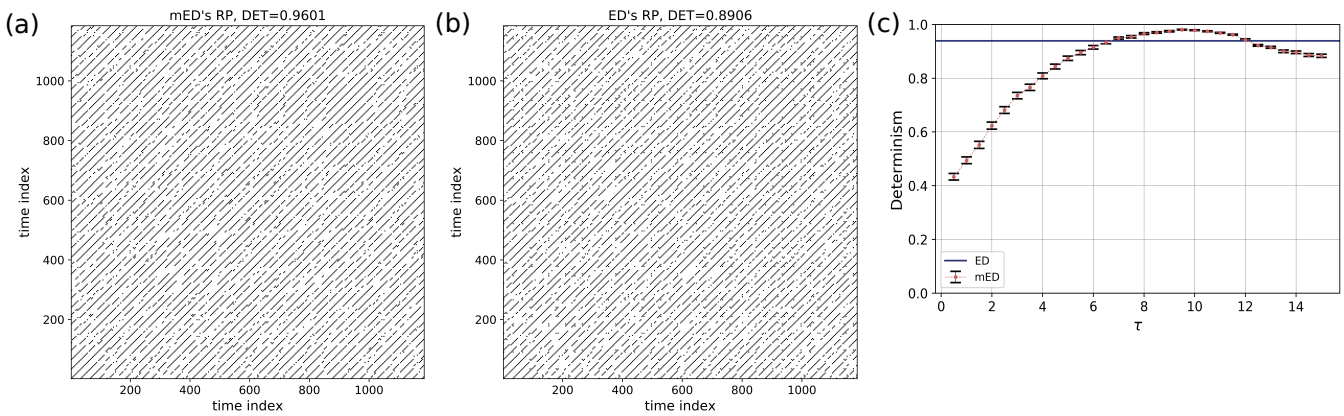
Figure 9. RP of a repeating Poisson process (Fig.7b) using (a) mED, (b) ED; (c) comparison of DET for 300 realisations using ED (blue horizontal line) and using mED for varying \tau in range 0 to 15.
