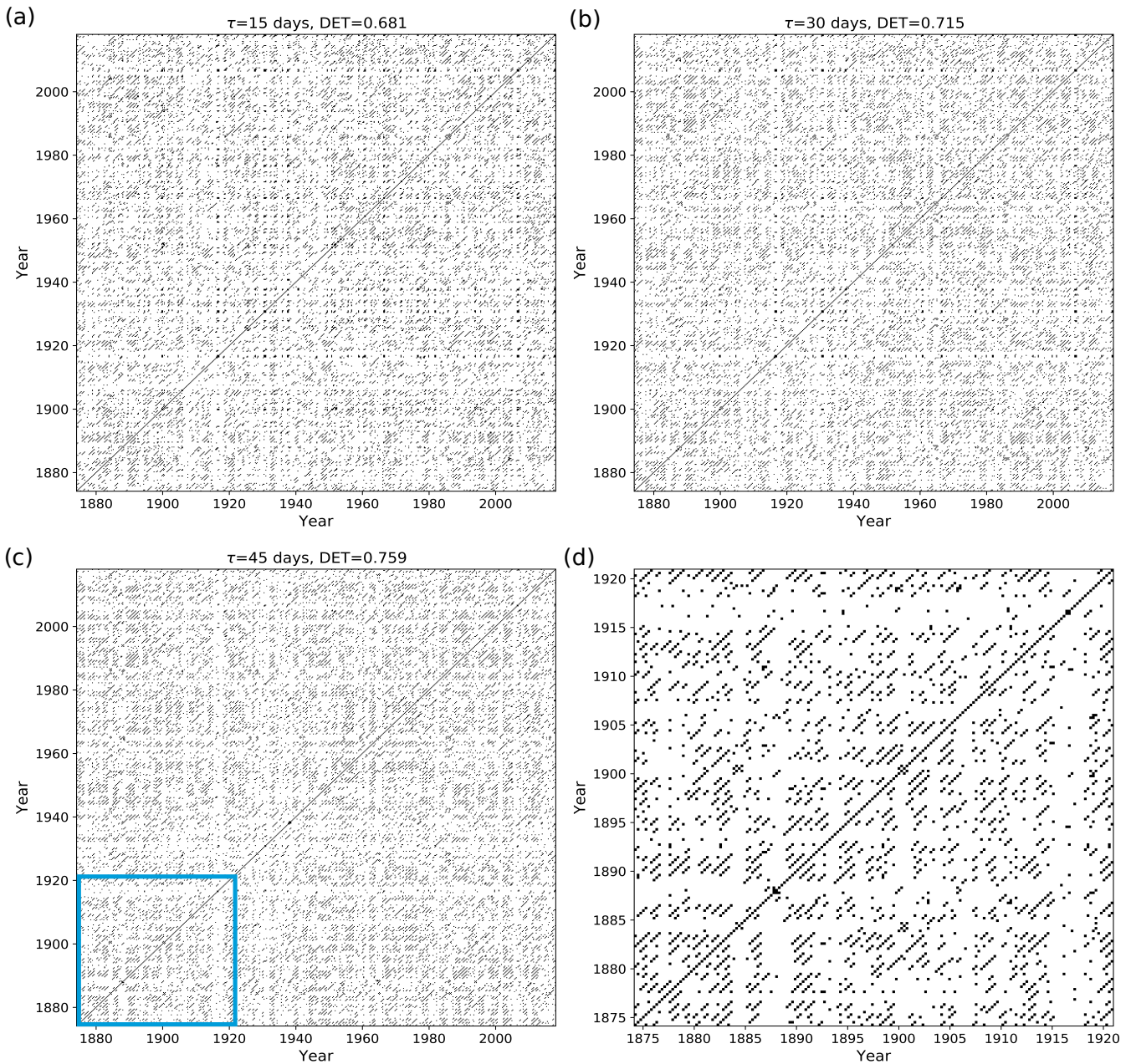
Figure 13. Recurrence plot of flood events using mED, window size = 1 year with 6 months overlap for delay \tau = (a) 15 days, (b) 30 days, and (c) 45 days; (d) zoom in image of the blue area of (c).
