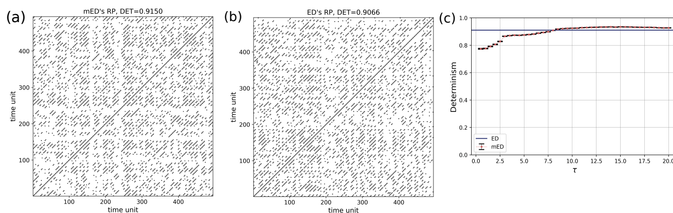
Figure 10. RP of Poisson process with periodical forcing (Fig.7c) using (a) mED, (b) ED; (c) comparison of DET for 300 realisations using ED (blue horizontal line) and using mED for varying \tau in range 0 to 20.
