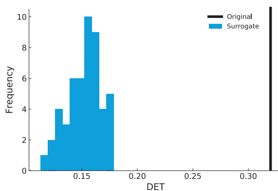
Figure 15. Distribution of DET value of surrogate data (blue) and the original DET value (black).
