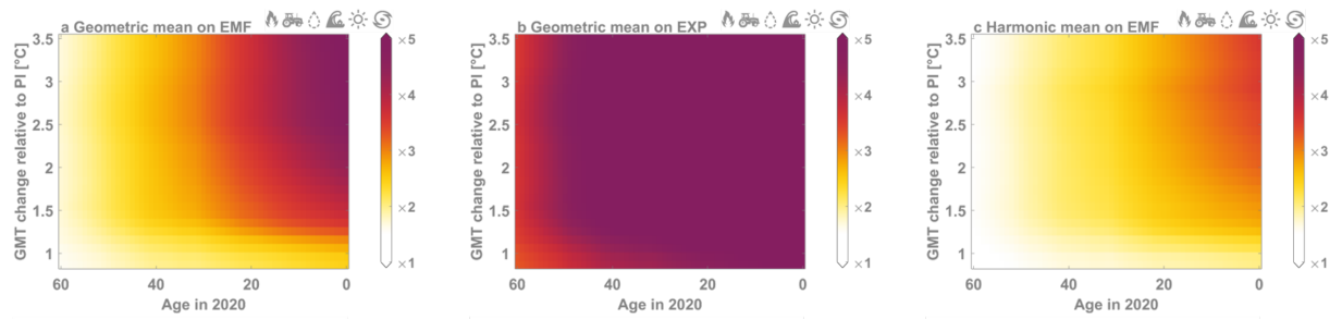
Supplementary Figure 2 | Cross-category lifetime exposure and influence of aggregation method on exposure sensitivity. (a) Same as fig. 2, but with exposure aggregated by computing the geometric mean across the exposure multiplication factor ( EMF ) per category, (b) Same as fig. 2, but with exposure aggregated by computing the geometric mean across the lifetime exposure ( EXP ), (c) Same as fig. 2, but with exposure aggregated by computing the harmonic mean across the EMF per category. We note that the second aggregation method (geometric mean on exposure) yields higher EMF values because the absence of events in one extreme event category results in zero cross-category exposure in a given country. As this occurs more frequently under pre-industrial control conditions, this leads to unrealistically low global-average pre-industrial control exposure values and hence artificially high EMF values.
