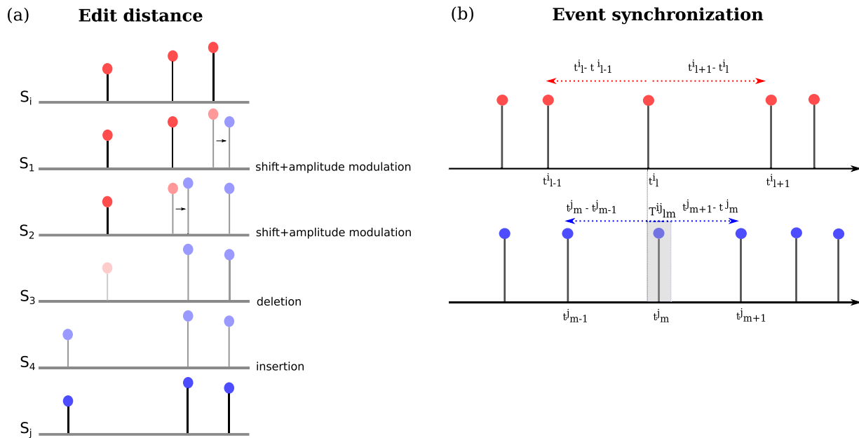
FIG. 2. Schematic illustration of (a) the edit distance method—segment S_i transformed to S_j by following the path from S_1 to S_4 operations; the final cost is obtained by minimizing all the possible combination. (b) The event synchronization— t_i^i and t_m^j are occurrence of events in the event series at grid point i and j , and T_{lm}^{ij} is the adaptive time lag.
