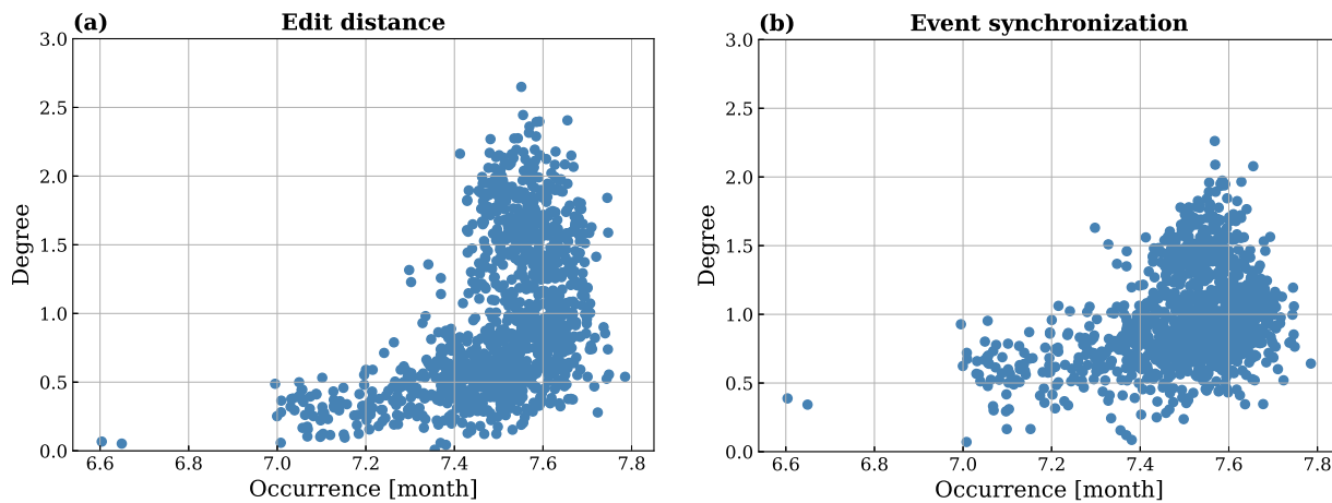
FIG. 8. Relationship between occurrences of peak precipitation and the connectedness between the grid points (degree) for the network constructed using (a) edit distance and (b) event synchronization.
