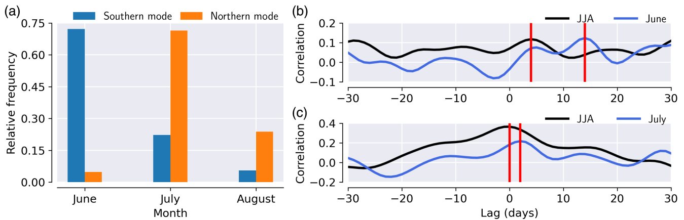
FIGURE 2 (a) The month-wise distribution of days with high ERE synchronization for the southern mode (ARB → SCN) and the northern mode (CMZ → NCN). Lead-lag correlations of low-pass filtered time series of spatially averaged daily numbers of extreme rainfall events (>90th percentile) in ARB and SCN (b, southern mode) and CMZ and NCN (c, northern mode) [Colour figure can be viewed at wileyonlinelibrary.com ]
