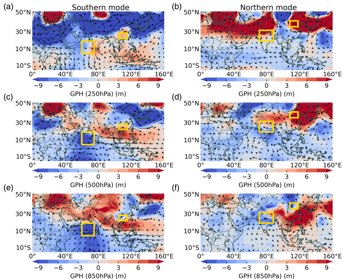
FIGURE 3 Composite anomalies of geopotential height at 250, 500 and 850 hPa, with respect to JJA climatology, based on the days of high ERE synchronization on Day 0, for southern (a, c, e) and northern (b, d, f) modes of ISM-EASM connection [Colour figure can be viewed at wileyonlinelibrary.com ]
