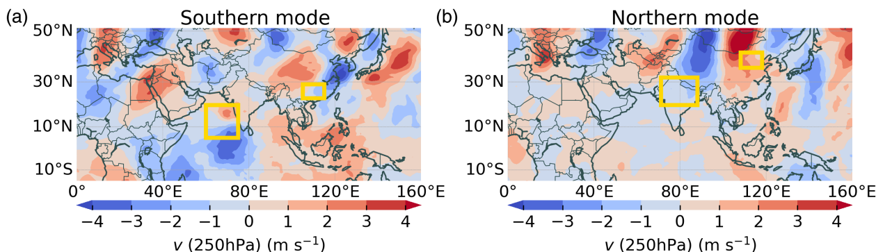
FIGURE 4 Composite anomalies of upper-level meridional wind component v at 250 hPa, with respect to JJA climatology, based on the days of high ERE synchronization on Day 0, for the southern (a) and northern (b) modes of the ISM–EASM connection [Colour figure can be viewed at wileyonlinelibrary.com ]
