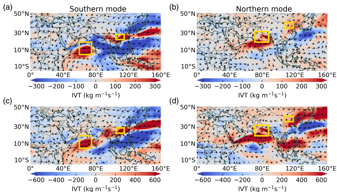
FIGURE 5 Aggregates of composite anomalies of vertically integrated water vapour flux, with respect to JJA climatology, for the southern mode for days (a) 0–4 and (c) 0–14. The same is also shown for the northern mode for days (b) 0–2 and (d) 0–14. Day 0 corresponds to days of high ERE synchronization for each mode of the ISM–EASM connection [Colour figure can be viewed at wileyonlinelibrary.com ]
