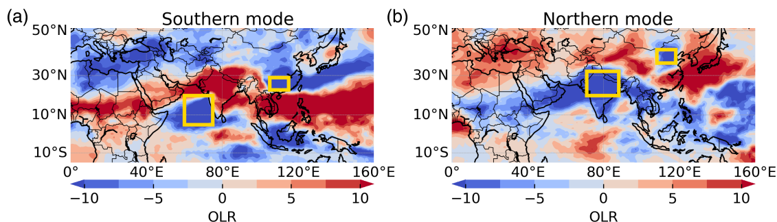
FIGURE 6 Composite anomalies of outgoing long-wave radiation, with respect to JJA climatology, based on the days of high synchronization on Day 0, for (a) southern and (b) northern modes of ISM–EASM connection [Colour figure can be viewed at wileyonlinelibrary.com ]
