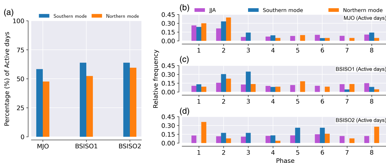
FIGURE 7 (a) Percentage of active (amplitude >1 ) MJO, BSISO1 and BSISO2 days among the specific days of high ERE synchronization for the southern and northern modes. MJO/BSISO phase distribution for days during the JJA season (for reference) and days of ERE synchronization for southern and northern modes which had active MJO (b), BSISO1 (c) and BSISO2 (d) [Colour figure can be viewed at wileyonlinelibrary.com ]
