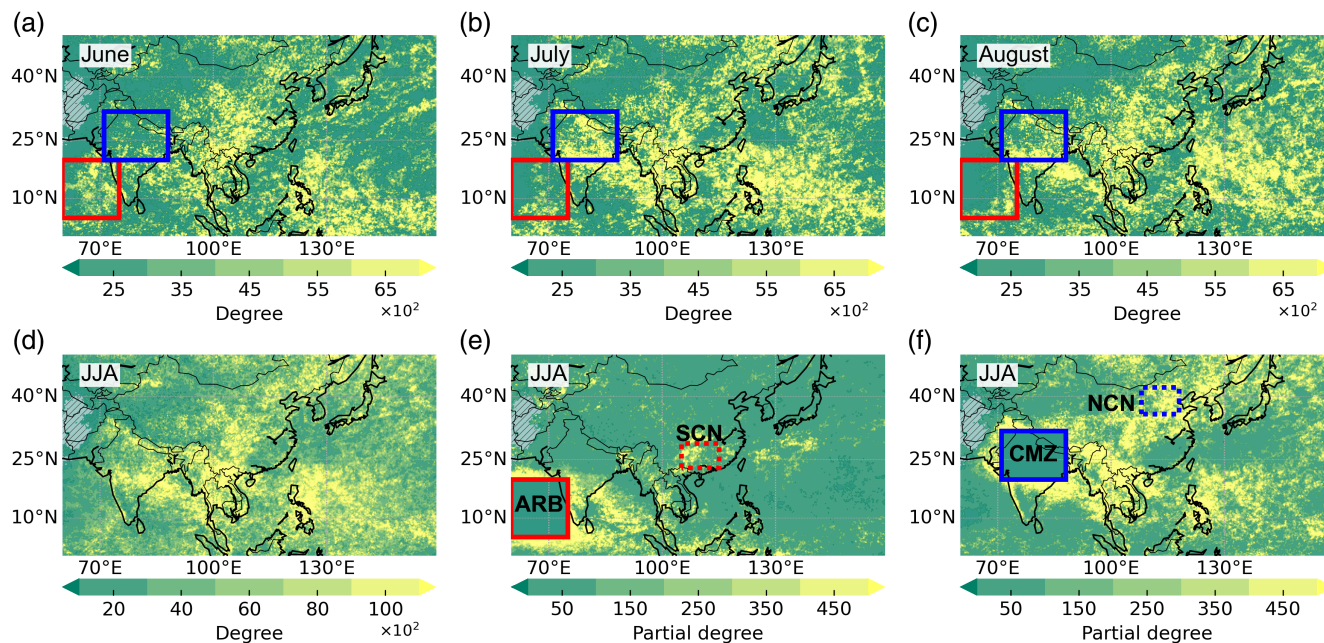
FIGURE 1 Monthly evolution of network degree for networks constructed for June (a), July (b) and August (c), respectively. The solid boxes are positioned at the Arabian Sea (ARB), and at the northern and central parts of India which is the core ISM zone (CMZ), respectively, to indicate noticeable changes in degree each month at different ISM regions. (d) Degree for the network constructed for the entire JJA season. (e, f) Partial degree for the regions, ARB (solid box: 5^{\circ} – 20^{\circ} N, 60^{\circ} – 75^{\circ} E) and CMZ (solid box: 20^{\circ} – 32^{\circ} N, 71^{\circ} – 88^{\circ} E), respectively, based on the network in (d) to indicate specific regions connected to each of them. From (e), it is seen that ARB has connections to southern China (SCN; dashed box: 23^{\circ} – 29^{\circ} N, 105^{\circ} – 115^{\circ} E) while from (f), CMZ is seen to be connected to parts in northern China (NCN; dashed box: 36^{\circ} – 42^{\circ} N, 108^{\circ} – 118^{\circ} E) [Colour figure can be viewed at wileyonlinelibrary.com ]
