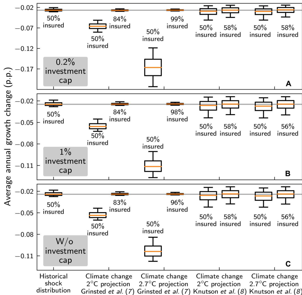
Fig. 5. Projected impacts of hurricanes on economic growth in 2° and 2.7°C worlds and the effectiveness of insurance as coping strategy. Average annual growth losses (relative to the corresponding unperturbed economies evolving on the BGPs) as obtained for the historical shock distribution (50% insurance coverage, period 1980–2014; first column), for Paris-compatible +2°C warming above preindustrial levels (second, third, sixth, and seventh columns), and for +2.7°C warming in compliance with current policies (fourth, fifth, eighth, and ninth columns) for reconstruction investment caps of 0.2% (A) (standard scenario), 1% (B), and without reconstruction investment cap (C). Climate change projections of growth losses are derived from two different methods to estimate climate change–induced changes in the return frequencies of hurricanes by Grinsted et al. (7) and Knutson et al. (8) (50% insurance coverage, second and fourth columns, respectively). In addition, for both estimates and warming levels, the insurance coverages that would be necessary to reduce growth losses to the historical level are shown (third, fifth, seventh, and ninth columns). Orange lines, boxes, and whiskers indicate median loss estimates as well as the 25th to 75th and 5th and 95th percentile ranges, respectively.
