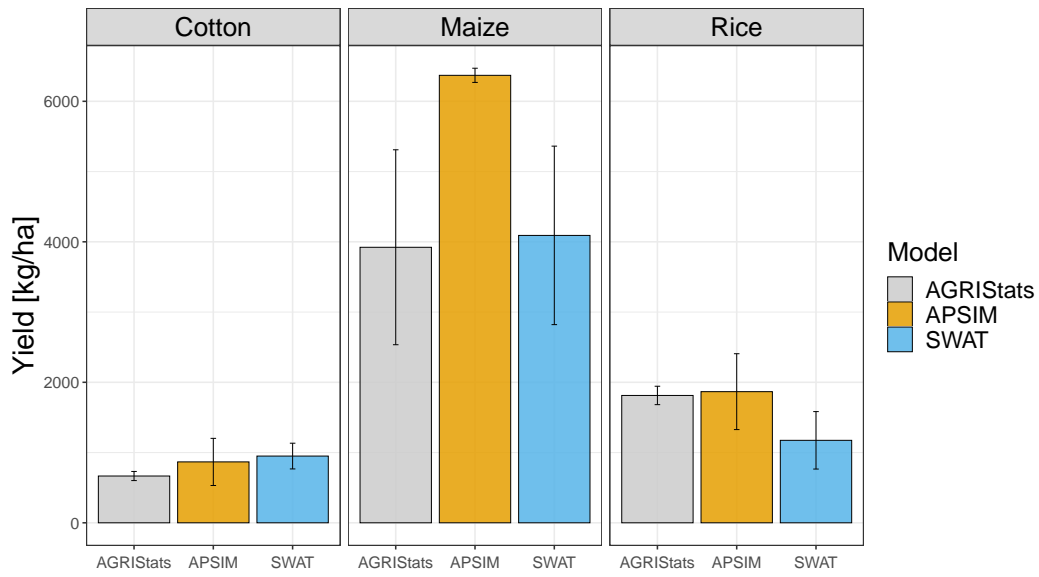
Figure S4. Validation of crop yield estimations
