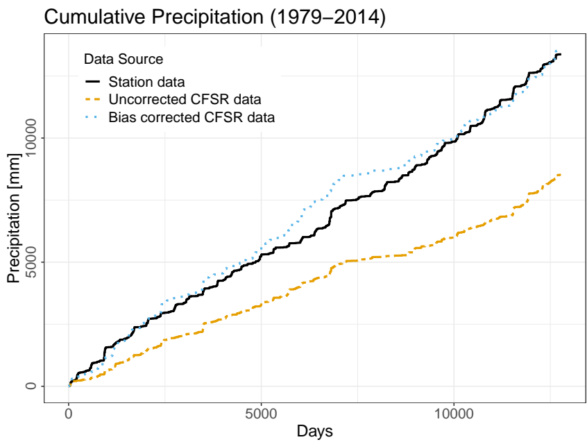
Figure S1. Results of precipitation bias correction procedure. Station data vs. uncorrected and bias corrected CFSR data
