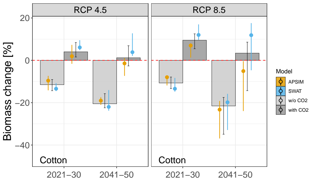
Figure S5. Simulated biomass changes for cotton
