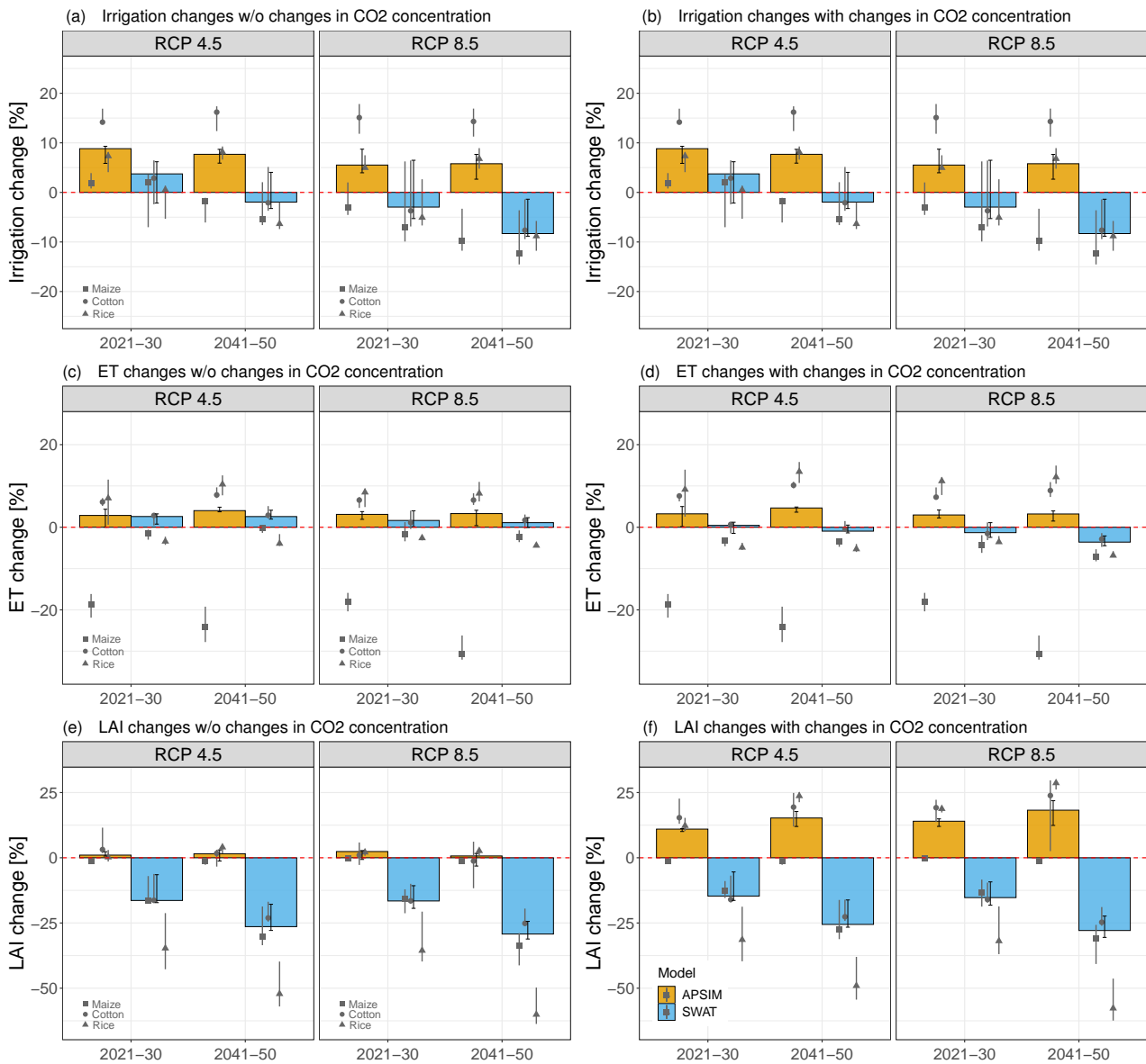
Figure S8. Simulated changes in irrigation demand, ET and LAI showing mean changes per model and for each crop type
