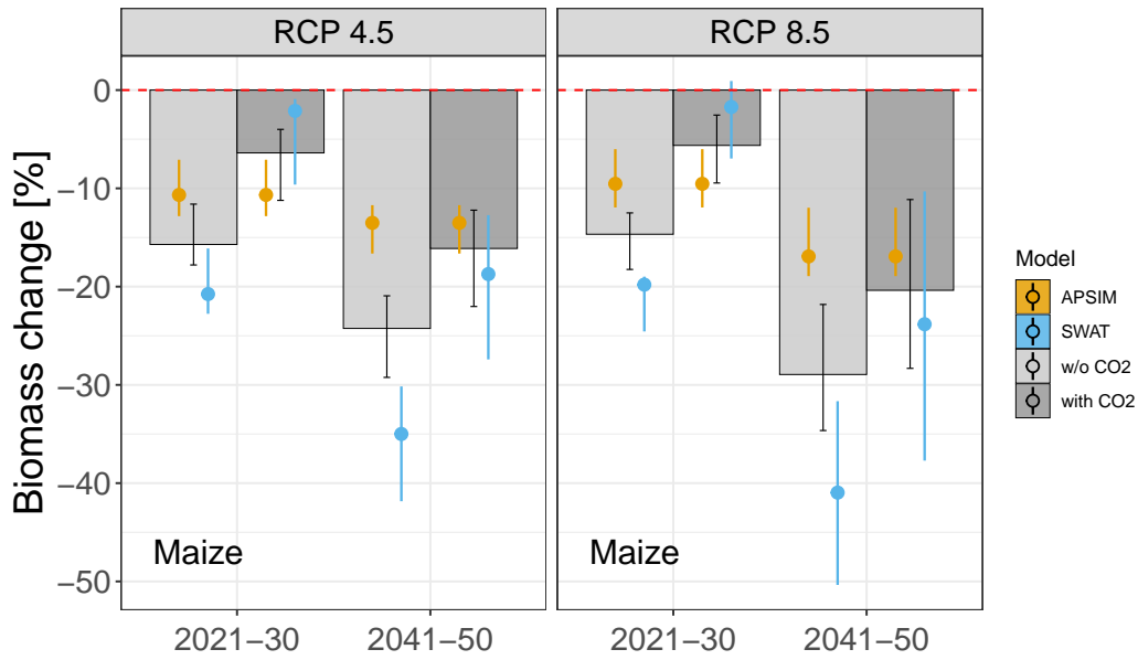
Figure S6. Simulated biomass changes for maize
