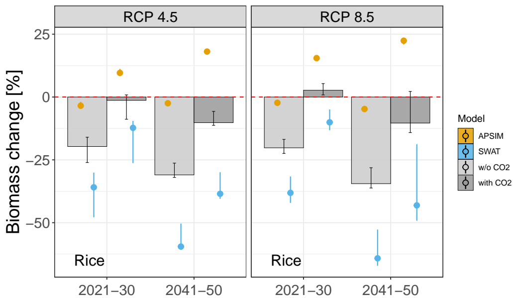
Figure S7. Simulated biomass changes for rice
