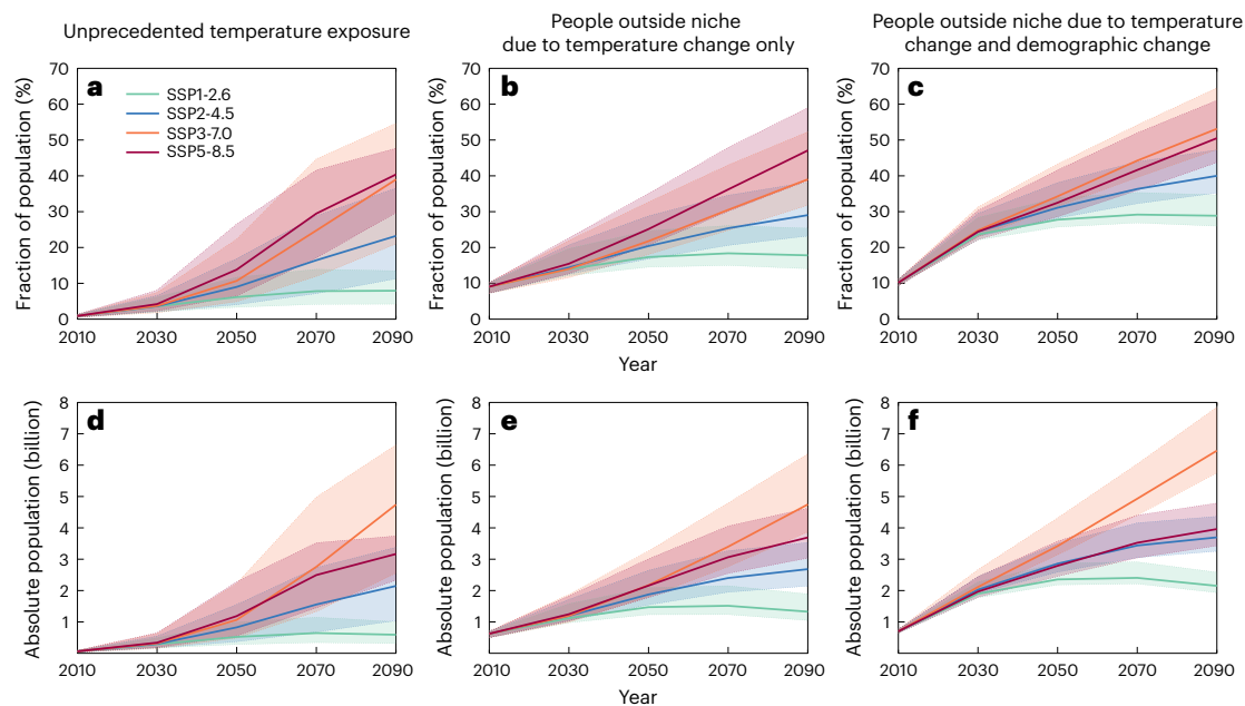
Fig. 2 | Population exposed outside of the temperature niche, following different SSPs. a–f. Fraction of population (%; a–c ) and absolute population (billion people; d–f ) exposed to unprecedented temperatures ( \text{MAT} \geq 29^\circ\text{C} ; a,d ), left outside the niche due to temperature change only ( b,e ) and left outside the niche due to temperature change and demographic change ( c,f ) for different
