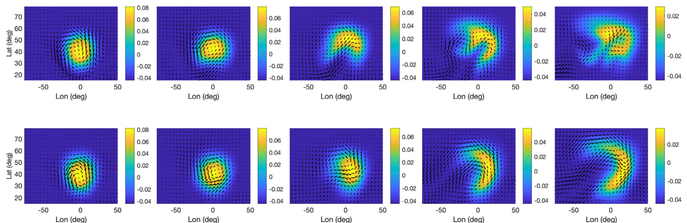
FIGURE 5 The evolution of buoyancy perturbations (represented in colors) in the lower layer and the corresponding velocity field (represented by arrows) during midlatitude adjustment in “dry” environment. The top and bottom rows show the results for barotropic and baroclinic configurations, respectively. The panels in each row display the evolution of the fields at 6, 13, 26, 43, and 65 days after the start of the simulation, arranged from left to right.
