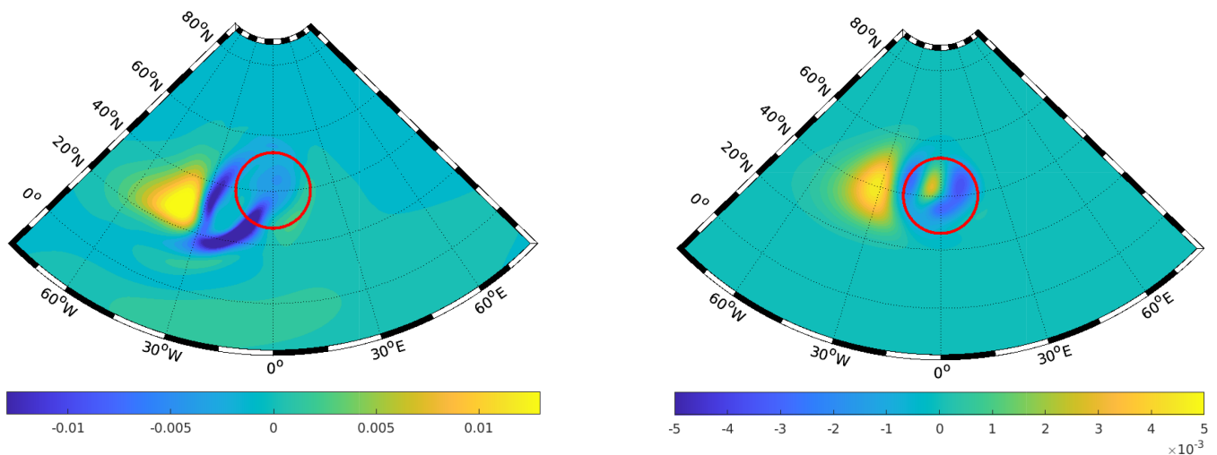
FIGURE 8 An asymmetric spatial distribution of the integrated energy density anomaly in the lower layer within a moist-convective environment was observed over a monthly duration for two distinct configurations: barotropic (left panel) and baroclinic (right panel). In both configurations, a strong buoyancy anomaly was utilized, and the initial temporal snapshot is denoted by the red circle, signifying the location of the large-scale, localized positive buoyancy anomaly.
