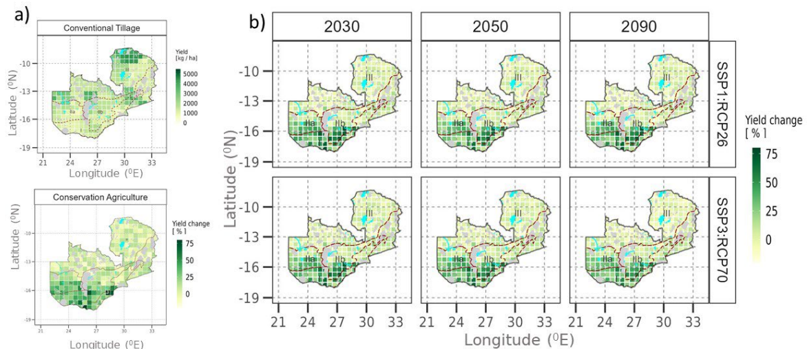
Figure 19: The grid-level spatial distribution map of a) projected sorghum yields in kg/ha under current climatic conditions with conventional tillage (top) and with conservation agriculture (bottom). b) shows changes in sorghum yield in % with conservation agriculture under the low emissions scenario SSP1-RCP2.6 (top) and the high emissions scenario SSP3-RCP7.0 (bottom) for periods of 20 years centered around 2030, 2050, and 2090
