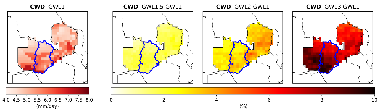
Figure 15: Average Crop Water Demand (CWD) between November and April in Zambia at a global warming level (GWL) of 1°C (left), representing current conditions, and the change from GWL 1°C to GWLs 1.5°C, 2°C and 3°C
