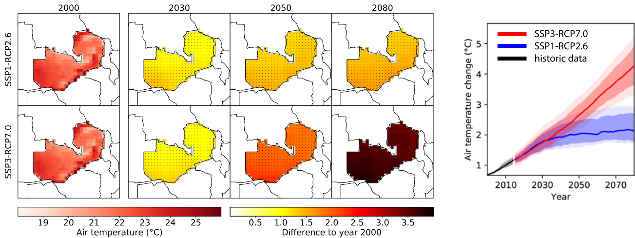
Figure 4: Projected temperature change in Zambia for SSP1-RCP2.6 and SSP3-RCP7.0
