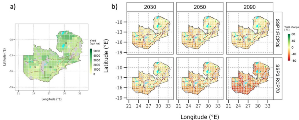
Figure 9: a) Current sorghum yields in kg/ha and b) projected future sorghum yield changes in% in Zambia at 0.5° grid under the low emissions scenario SSP1-RCP2.6 (top row) and the high emissions scenario SSP3-RCP7.0 (bottom row) for periods of 20 years centered around 2030, 2050, and 2090; The projections were calculated based on the process-based crop model DSSAT (see Box 4)
