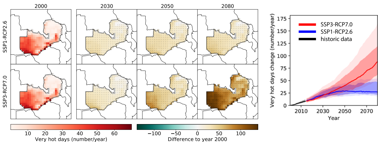
Figure 5: Projected change in the number of very hot days per year under SSP1-RCP2.6 and SSP3-RCP7.0; very hot days refer to days with a maximum near-surface air temperature above 35°C
