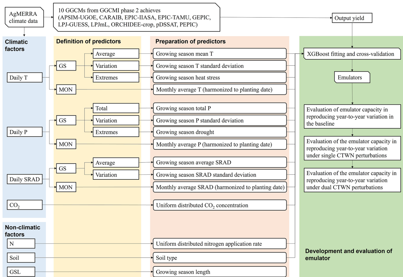
Figure 1. Overall framework of emulator development for GGCMs. Each GGCM–crop combination was calibrated as an emulator independently. T : temperature, processed separately for daily maximum and minimum temperatures; P : precipitation; SRAD: solar radiation, N: nitrogen; soil: soil properties. When developing irrigated yield emulator, precipitation-related predictors are excluded.
