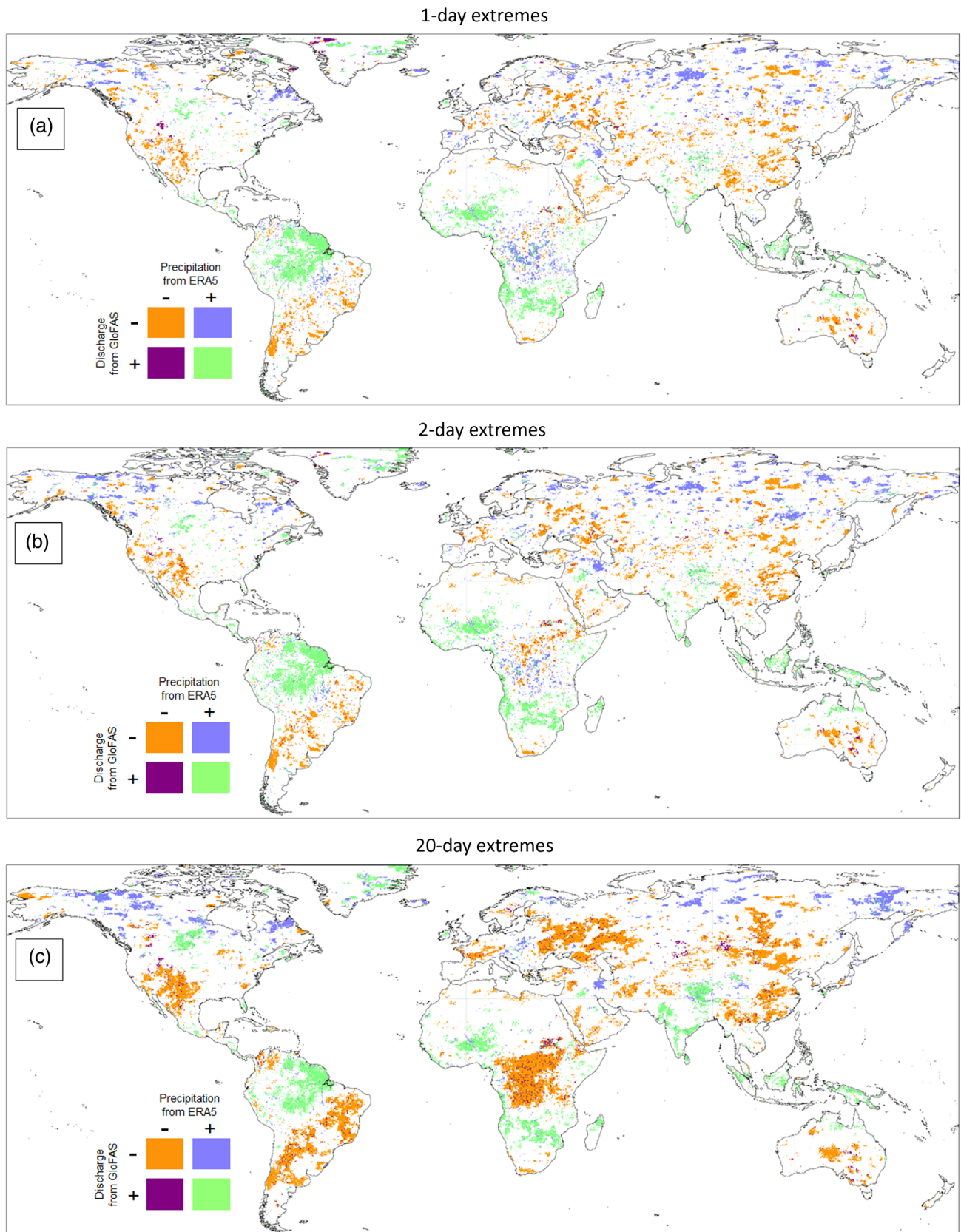
FIGURE 3 Convergence and divergence in the sign of significant trends in extremes of precipitation and of discharge, for period 1979–2020. This is calculated for annual maximum cumulative values of precipitation and of discharge during consecutive periods of 1-day (panel a), 2-day (b), and 20-day (c). Colors show where precipitation and discharge extremes both increase (green), both decrease (orange), where precipitation increases while discharge decreases (blue), and where precipitation decreases while discharge increases (purple). Precipitation data are from ERA5 (Hersbach et al., 2020), and discharge data are from GloFAS (Harrigan et al., 2020). Trend significance is assessed with the Mann-Kendall test.
