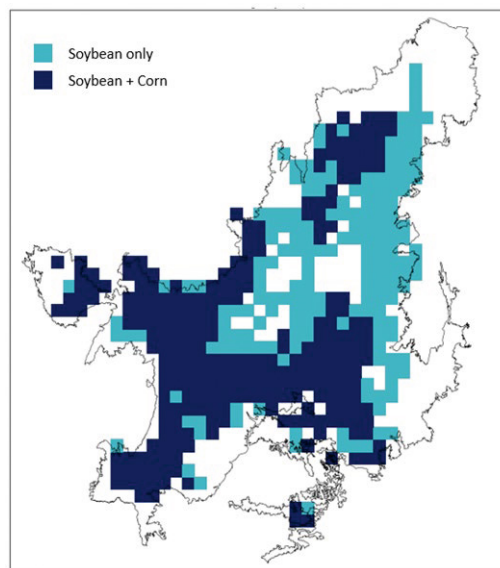
Figure 3. Cerrado areas with either single-crop (soybean only) or double-crop (soybean followed by corn as a second crop).
