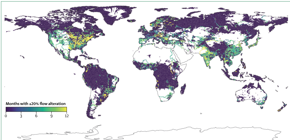
Figure 16: Months per year in which modelled observed monthly surface water flows differ by >20% from modelled pre-industrial flows Such flow alterations (ie, outside the Earth-system boundary), which result from meeting the needs and aspirations of people, lead to a breakdown in function of the aquatic ecosystem, causing reduced fisheries production and the loss of other ecosystem services, which affects human health and livelihoods.
